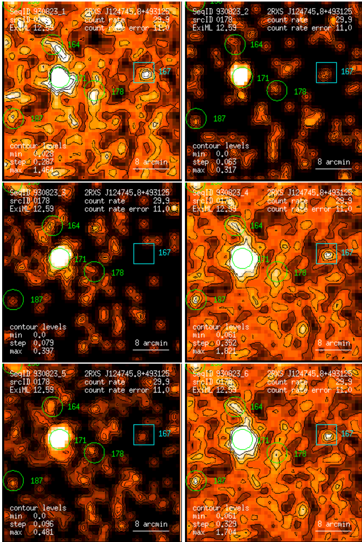
Figure 178: RASS 930823: detection 0178: band rate images, Gaussian filter: (1) PSPC channels 11 – 41, (2) 52 – 90, (3) 91 – 201, (4) 11 – 235, (5) 52 – 201, (6) 11 – 201. Broad band rates in counts/ks. Band rate contour levels in counts/ks/arcmin 2 .
