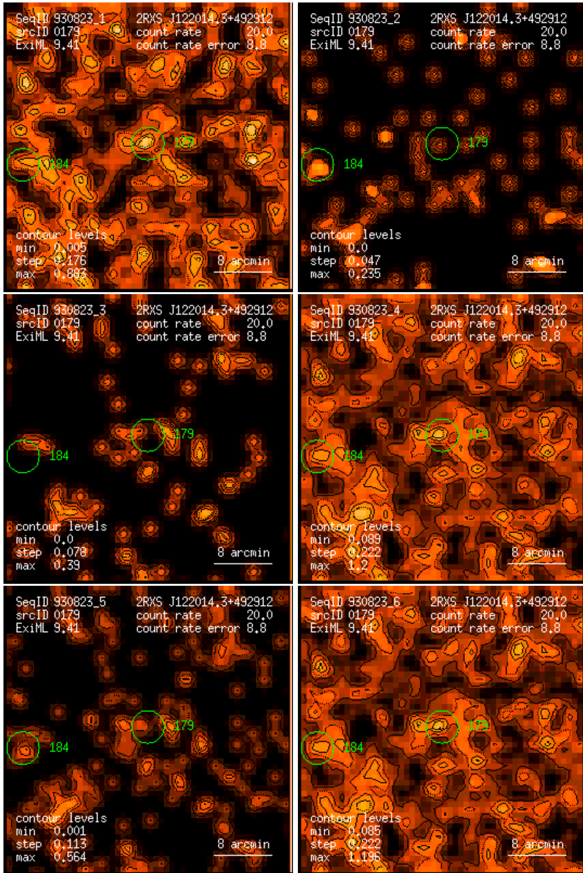
Figure 179: RASS 930823: detection 0179: band rate images, Gaussian filter: (1) PSPC channels 11 – 41, (2) 52 – 90, (3) 91 – 201, (4) 11 – 235, (5) 52 – 201, (6) 11 – 201. Broad band rates in counts/ks. Band rate contour levels in counts/ks/arcmin 2 .
