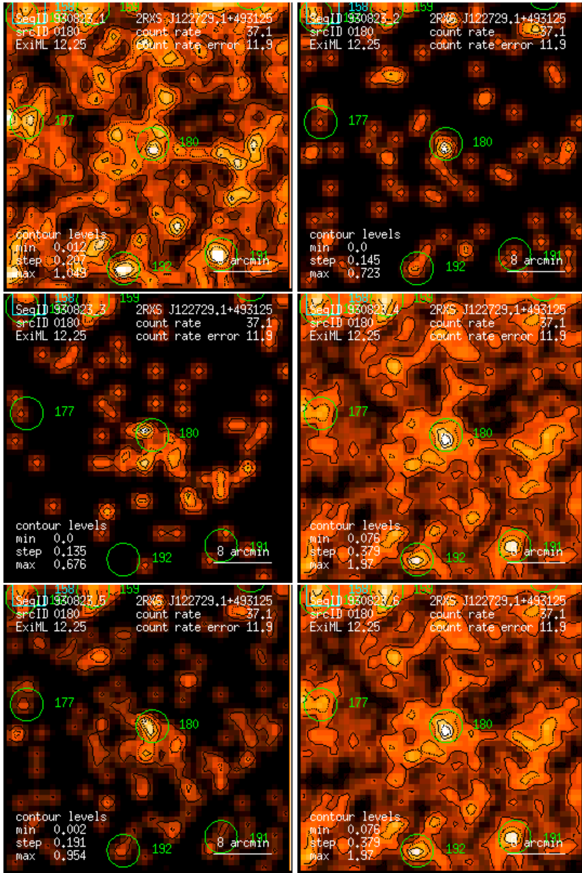
Figure 180: RASS 930823: detection 0180: band rate images, Gaussian filter: (1) PSPC channels 11 – 41, (2) 52 – 90, (3) 91 – 201, (4) 11 – 235, (5) 52 – 201, (6) 11 – 201. Broad band rates in counts/ks. Band rate contour levels in counts/ks/arcmin 2 .
