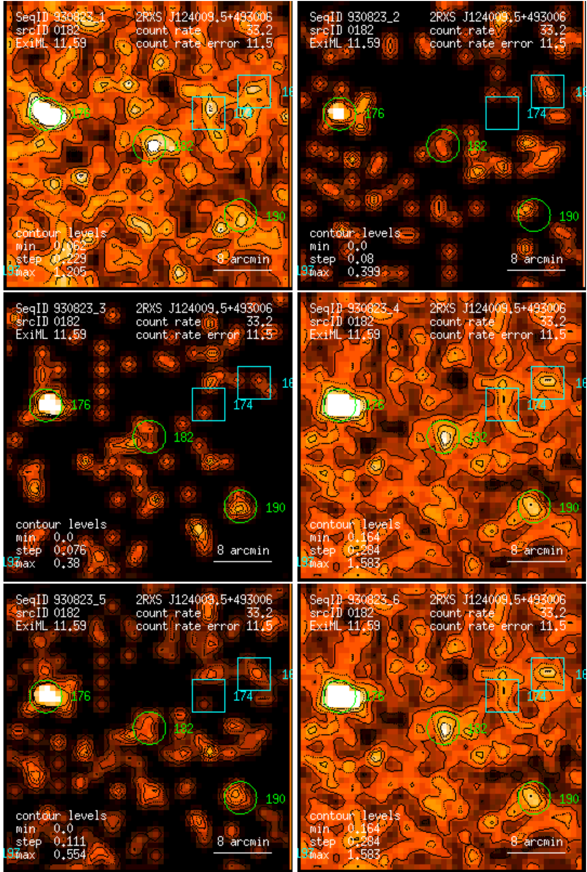
Figure 182: RASS 930823: detection 0182: band rate images, Gaussian filter: (1) PSPC channels 11 – 41, (2) 52 – 90, (3) 91 – 201, (4) 11 – 235, (5) 52 – 201, (6) 11 – 201. Broad band rates in counts/ks. Band rate contour levels in counts/ks/arcmin 2 .
