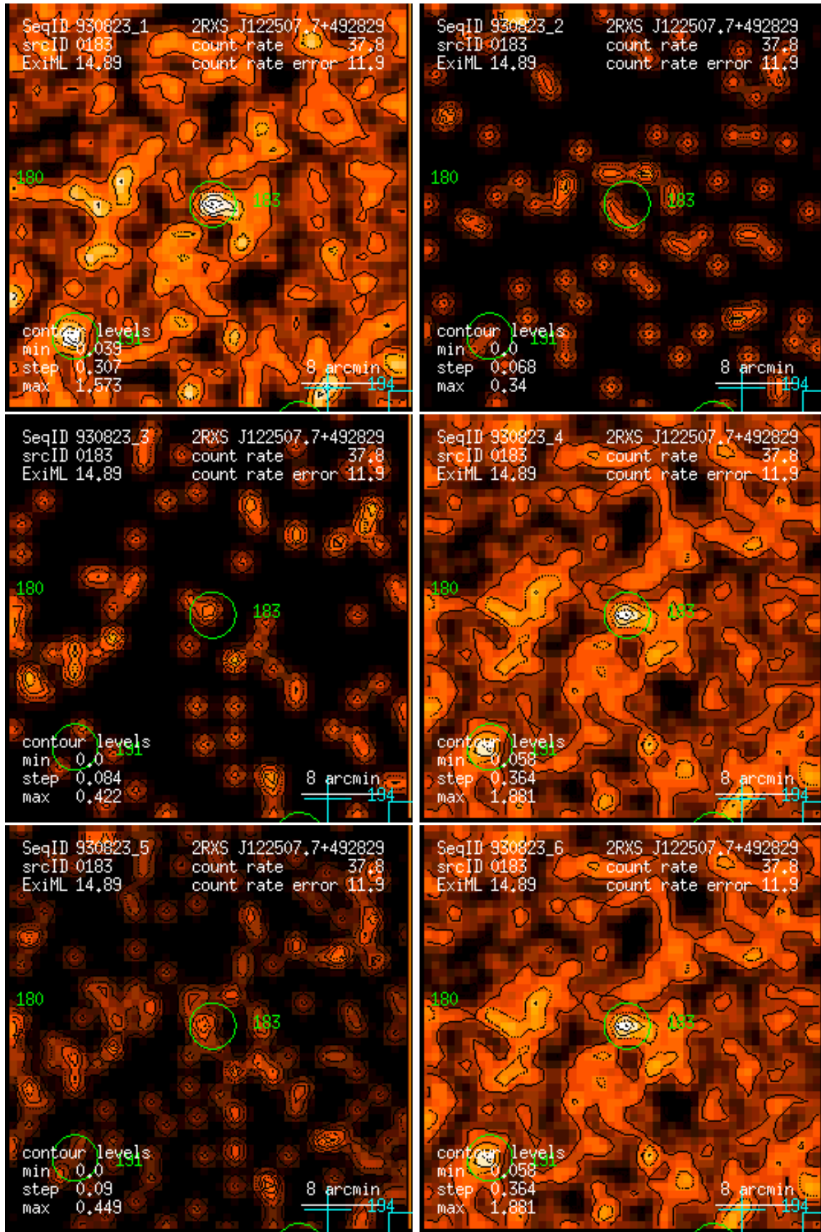
Figure 183: RASS 930823: detection 0183: band rate images, Gaussian filter: (1) PSPC channels 11 – 41, (2) 52 – 90, (3) 91 – 201, (4) 11 – 235, (5) 52 – 201, (6) 11 – 201. Broad band rates in counts/ks. Band rate contour levels in counts/ks/arcmin 2 .
