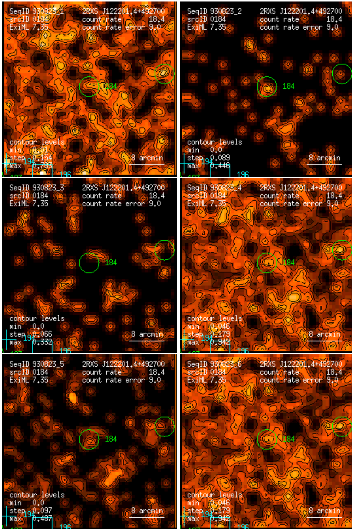
Figure 184: RASS 930823: detection 0184: band rate images, Gaussian filter: (1) PSPC channels 11 – 41, (2) 52 – 90, (3) 91 – 201, (4) 11 – 235, (5) 52 – 201, (6) 11 – 201. Broad band rates in counts/ks. Band rate contour levels in counts/ks/arcmin 2 .
