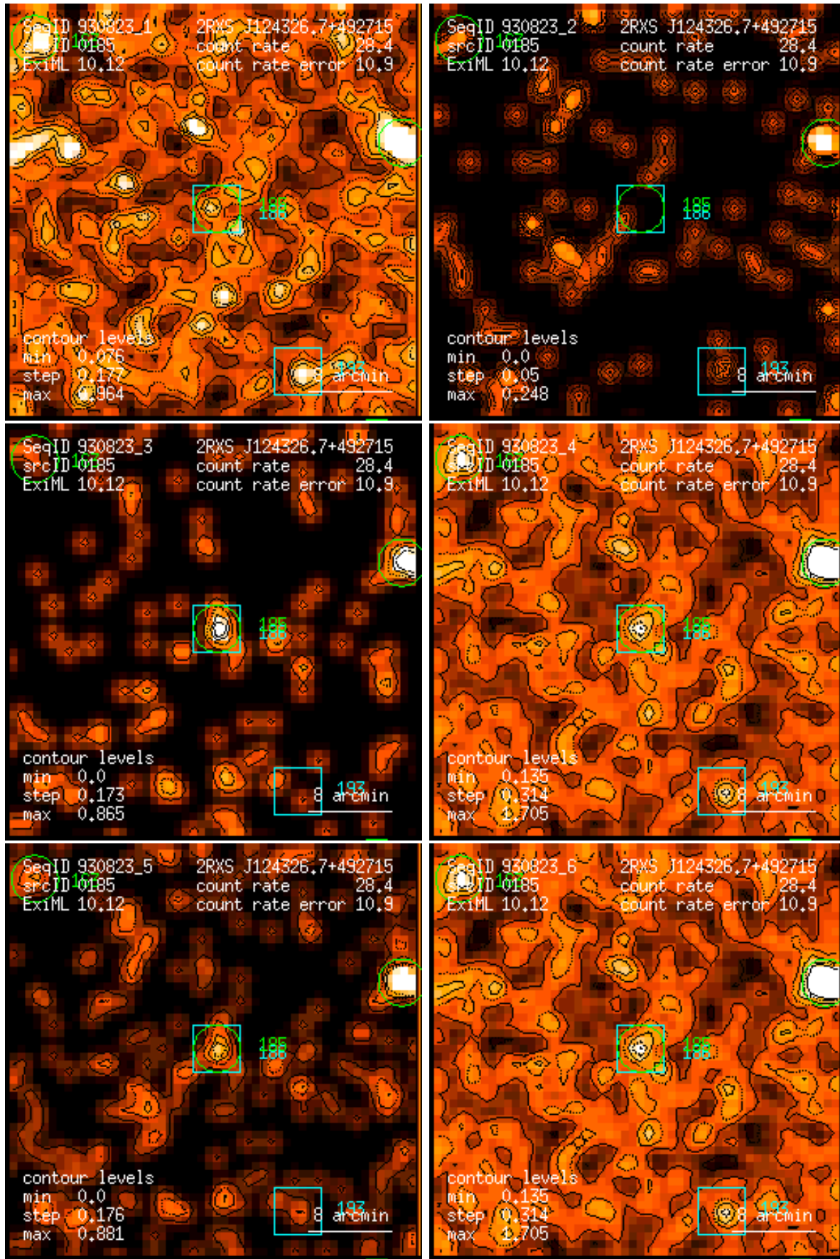
Figure 185: RASS 930823: detection 0185: band rate images, Gaussian filter: (1) PSPC channels 11 – 41, (2) 52 – 90, (3) 91 – 201, (4) 11 – 235, (5) 52 – 201, (6) 11 – 201. Broad band rates in counts/ks. Band rate contour levels in counts/ks/arcmin 2 .
