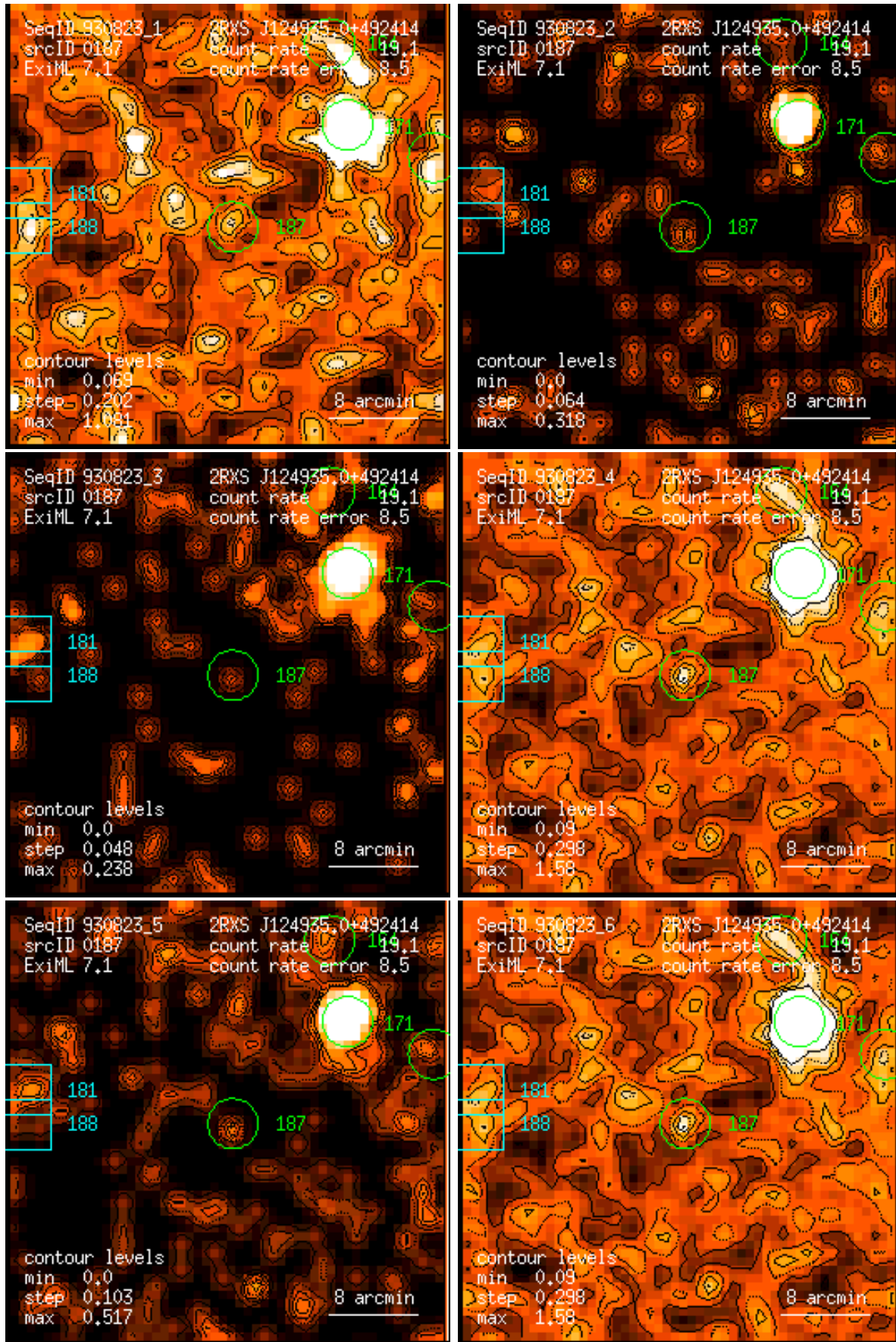
Figure 187: RASS 930823: detection 0187: band rate images, Gaussian filter: (1) PSPC channels 11 – 41, (2) 52 – 90, (3) 91 – 201, (4) 11 – 235, (5) 52 – 201, (6) 11 – 201. Broad band rates in counts/ks. Band rate contour levels in counts/ks/arcmin 2 .
