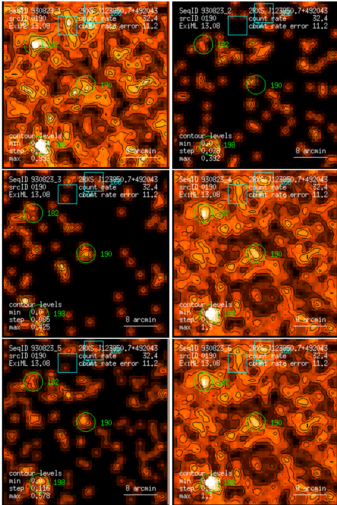
Figure 190: RASS 930823: detection 0190: band rate images, Gaussian filter: (1) PSPC channels 11 – 41, (2) 52 – 90, (3) 91 – 201, (4) 11 – 235, (5) 52 – 201, (6) 11 – 201. Broad band rates in counts/ks. Band rate contour levels in counts/ks/arcmin 2 .
