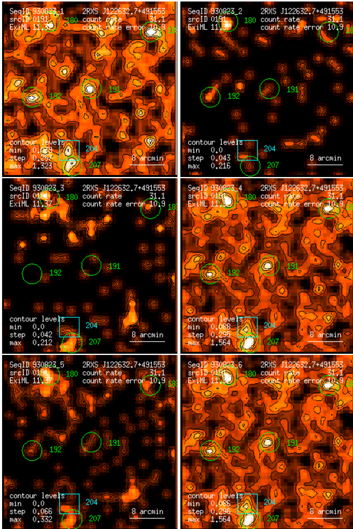
Figure 191: RASS 930823: detection 0191: band rate images, Gaussian filter: (1) PSPC channels 11 – 41, (2) 52 – 90, (3) 91 – 201, (4) 11 – 235, (5) 52 – 201, (6) 11 – 201. Broad band rates in counts/ks. Band rate contour levels in counts/ks/arcmin 2 .
