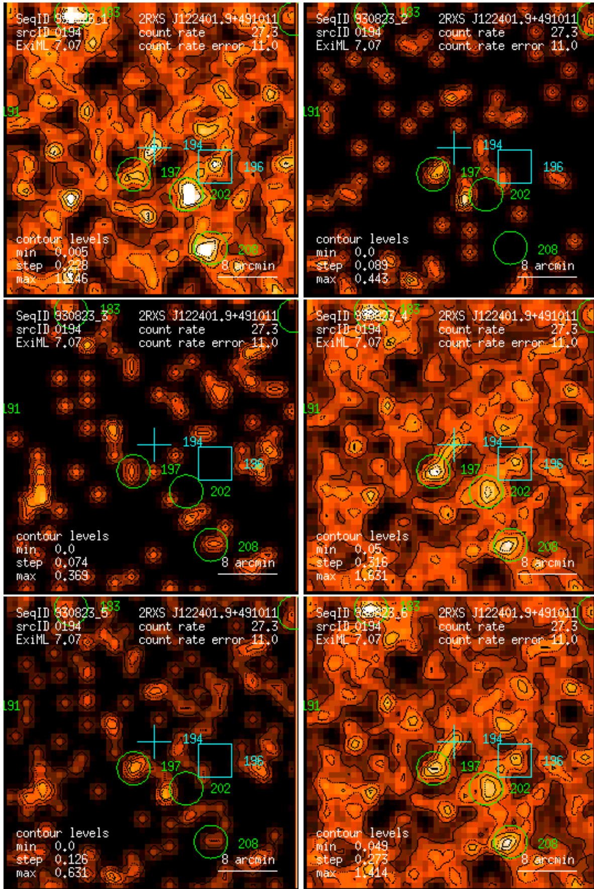
Figure 194: RASS 930823: detection 0194: band rate images, Gaussian filter: (1) PSPC channels 11 – 41, (2) 52 – 90, (3) 91 – 201, (4) 11 – 235, (5) 52 – 201, (6) 11 – 201. Broad band rates in counts/ks. Band rate contour levels in counts/ks/arcmin 2 .
