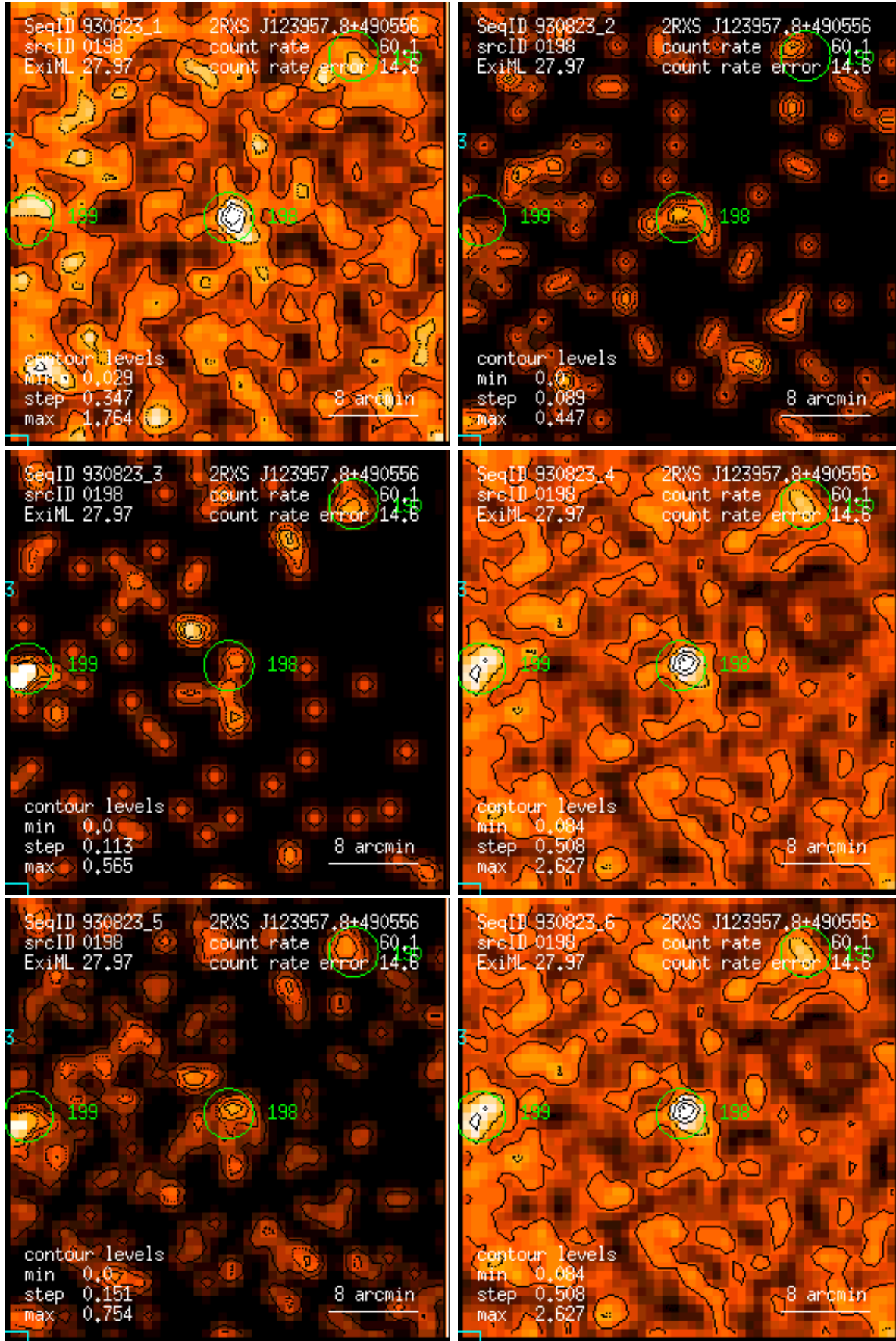
Figure 198: RASS 930823: detection 0198: band rate images, Gaussian filter: (1) PSPC channels 11 – 41, (2) 52 – 90, (3) 91 – 201, (4) 11 – 235, (5) 52 – 201, (6) 11 – 201. Broad band rates in counts/ks. Band rate contour levels in counts/ks/arcmin 2 .
