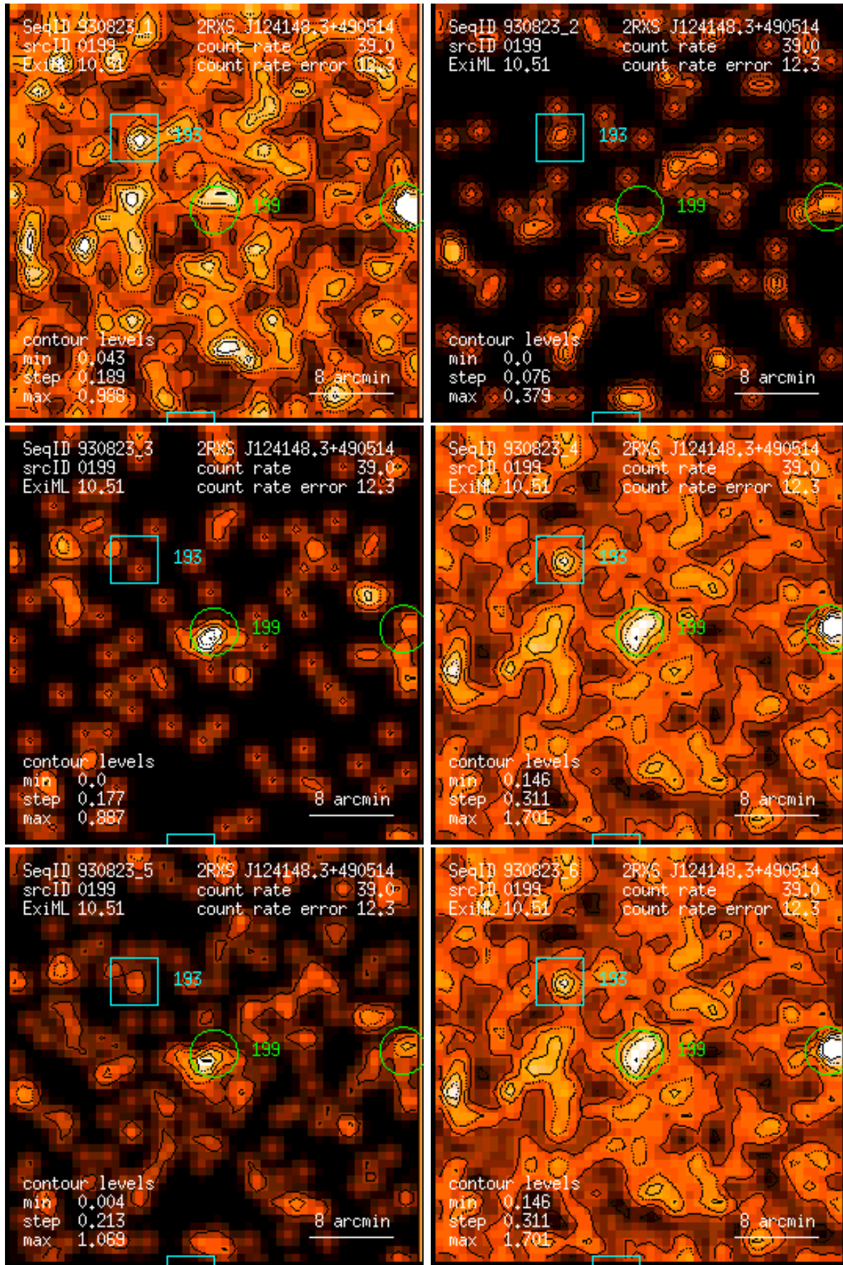
Figure 199: RASS 930823: detection 0199: band rate images, Gaussian filter: (1) PSPC channels 11 – 41, (2) 52 – 90, (3) 91 – 201, (4) 11 – 235, (5) 52 – 201, (6) 11 – 201. Broad band rates in counts/ks. Band rate contour levels in counts/ks/arcmin 2 .
