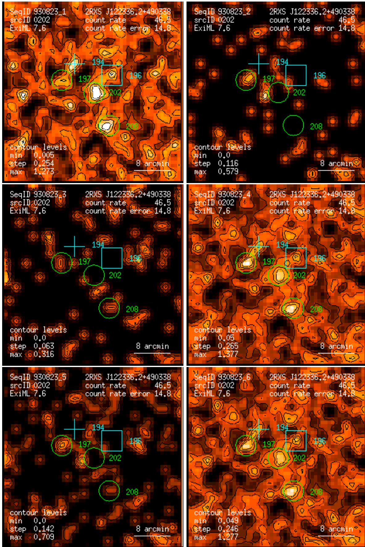
Figure 202: RASS 930823: detection 0202: band rate images, Gaussian filter: (1) PSPC channels 11 – 41, (2) 52 – 90, (3) 91 – 201, (4) 11 – 235, (5) 52 – 201, (6) 11 – 201. Broad band rates in counts/ks. Band rate contour levels in counts/ks/arcmin 2 .
