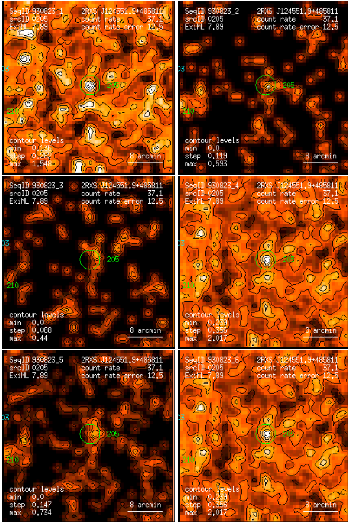
Figure 205: RASS 930823: detection 0205: band rate images, Gaussian filter: (1) PSPC channels 11 – 41, (2) 52 – 90, (3) 91 – 201, (4) 11 – 235, (5) 52 – 201, (6) 11 – 201. Broad band rates in counts/ks. Band rate contour levels in counts/ks/arcmin 2 .
