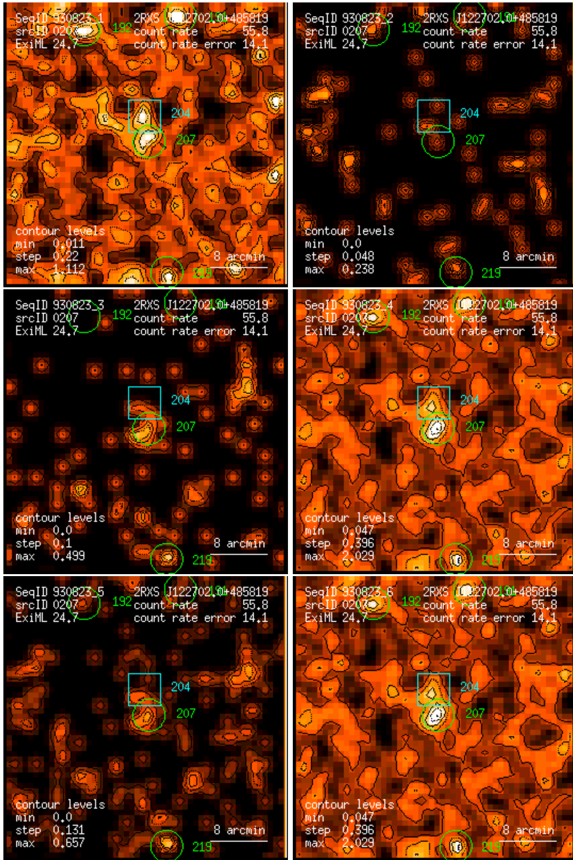
Figure 207: RASS 930823: detection 0207: band rate images, Gaussian filter: (1) PSPC channels 11 – 41, (2) 52 – 90, (3) 91 – 201, (4) 11 – 235, (5) 52 – 201, (6) 11 – 201. Broad band rates in counts/ks. Band rate contour levels in counts/ks/arcmin 2 .
