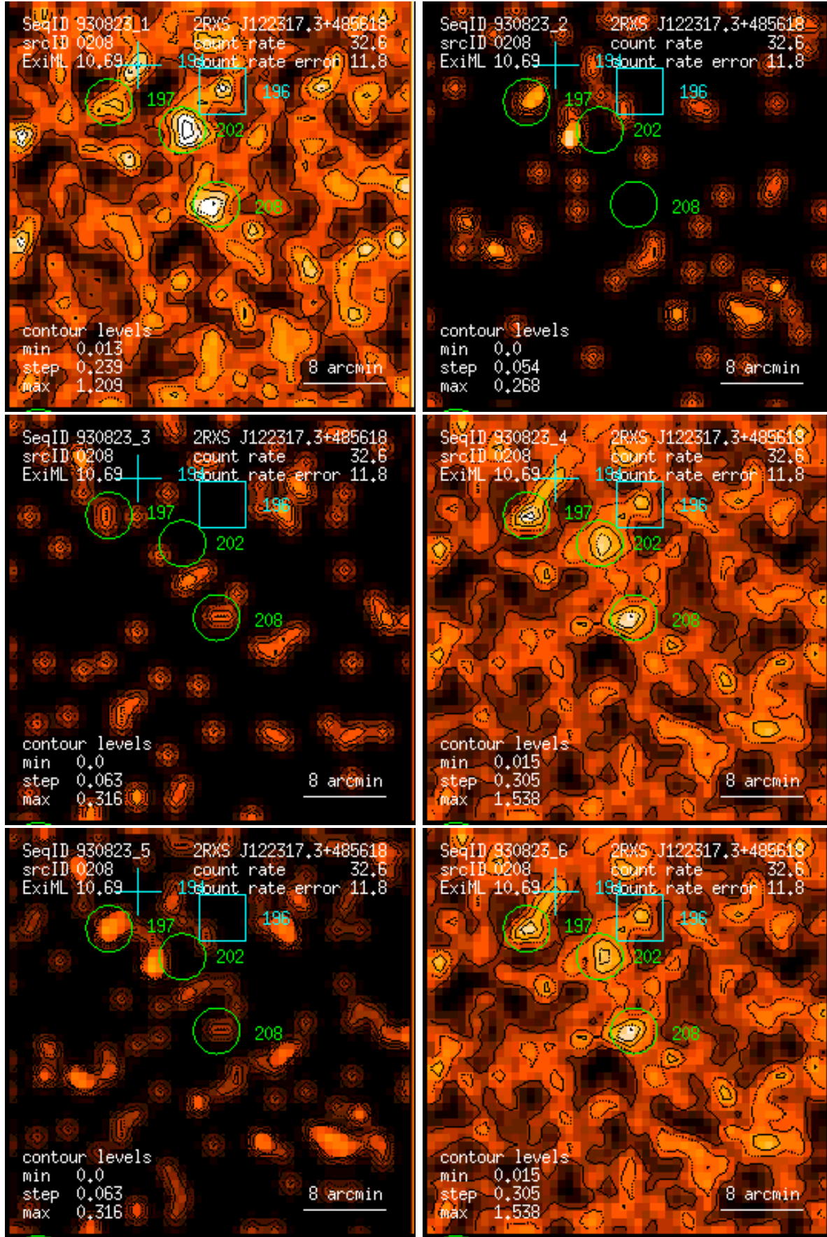
Figure 208: RASS 930823: detection 0208: band rate images, Gaussian filter: (1) PSPC channels 11 – 41, (2) 52 – 90, (3) 91 – 201, (4) 11 – 235, (5) 52 – 201, (6) 11 – 201. Broad band rates in counts/ks. Band rate contour levels in counts/ks/arcmin 2 .
