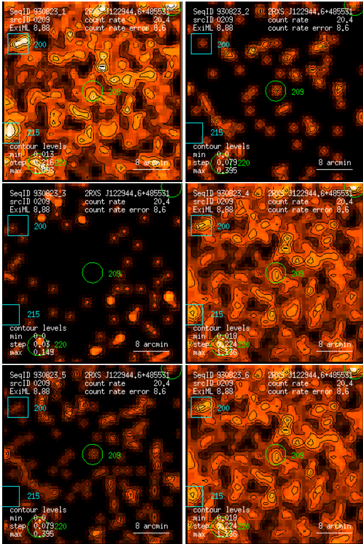
Figure 209: RASS 930823: detection 0209: band rate images, Gaussian filter: (1) PSPC channels 11 – 41, (2) 52 – 90, (3) 91 – 201, (4) 11 – 235, (5) 52 – 201, (6) 11 – 201. Broad band rates in counts/ks. Band rate contour levels in counts/ks/arcmin 2 .
