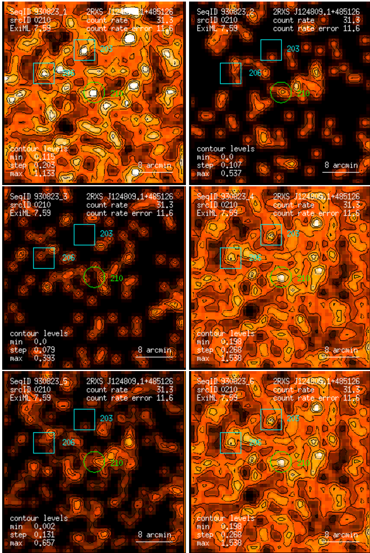
Figure 210: RASS 930823: detection 0210: band rate images, Gaussian filter: (1) PSPC channels 11 – 41, (2) 52 – 90, (3) 91 – 201, (4) 11 – 235, (5) 52 – 201, (6) 11 – 201. Broad band rates in counts/ks. Band rate contour levels in counts/ks/arcmin 2 .
