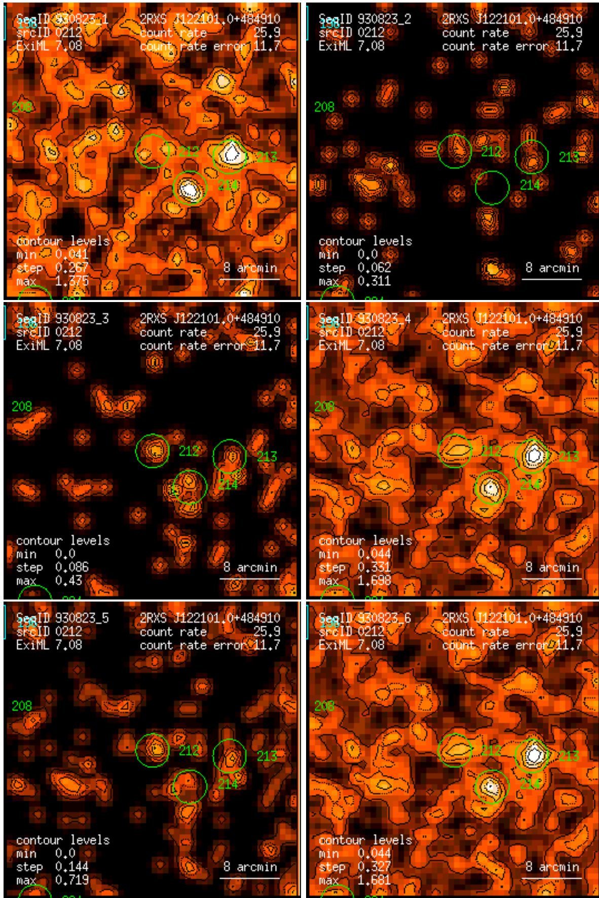
Figure 212: RASS 930823: detection 0212: band rate images, Gaussian filter: (1) PSPC channels 11 – 41, (2) 52 – 90, (3) 91 – 201, (4) 11 – 235, (5) 52 – 201, (6) 11 – 201. Broad band rates in counts/ks. Band rate contour levels in counts/ks/arcmin 2 .
