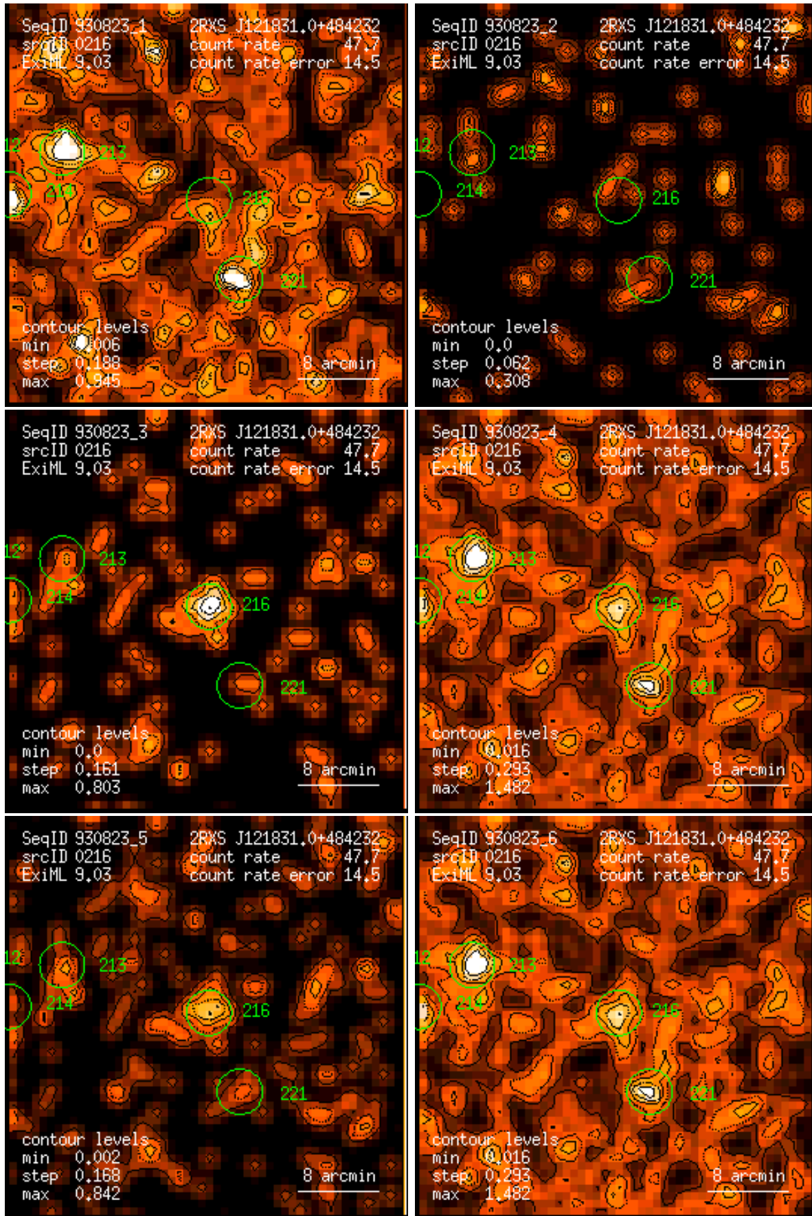
Figure 216: RASS 930823: detection 0216: band rate images, Gaussian filter: (1) PSPC channels 11 – 41, (2) 52 – 90, (3) 91 – 201, (4) 11 – 235, (5) 52 – 201, (6) 11 – 201. Broad band rates in counts/ks. Band rate contour levels in counts/ks/arcmin 2 .
