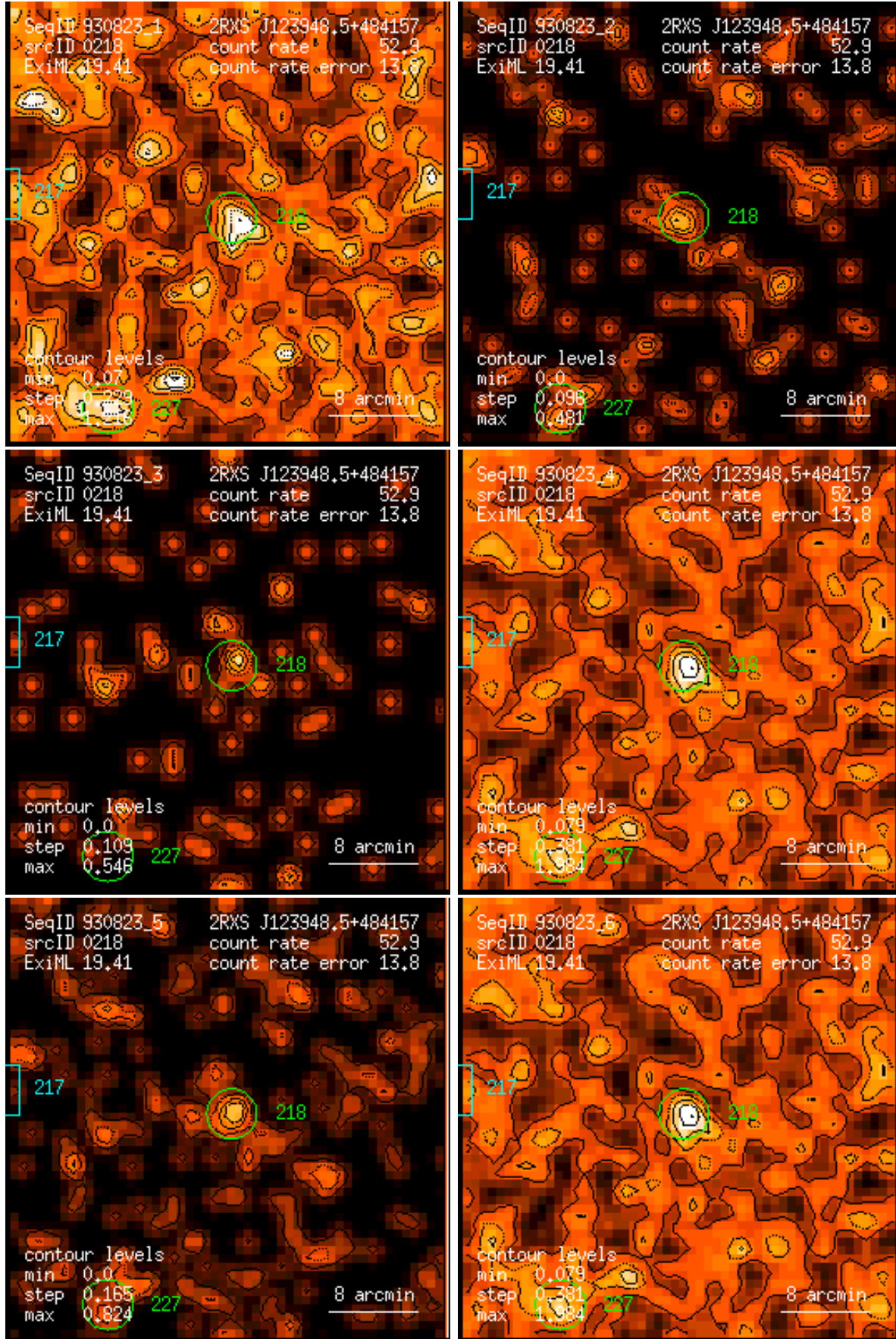
Figure 218: RASS 930823: detection 0218: band rate images, Gaussian filter: (1) PSPC channels 11 – 41, (2) 52 – 90, (3) 91 – 201, (4) 11 – 235, (5) 52 – 201, (6) 11 – 201. Broad band rates in counts/ks. Band rate contour levels in counts/ks/arcmin 2 .
