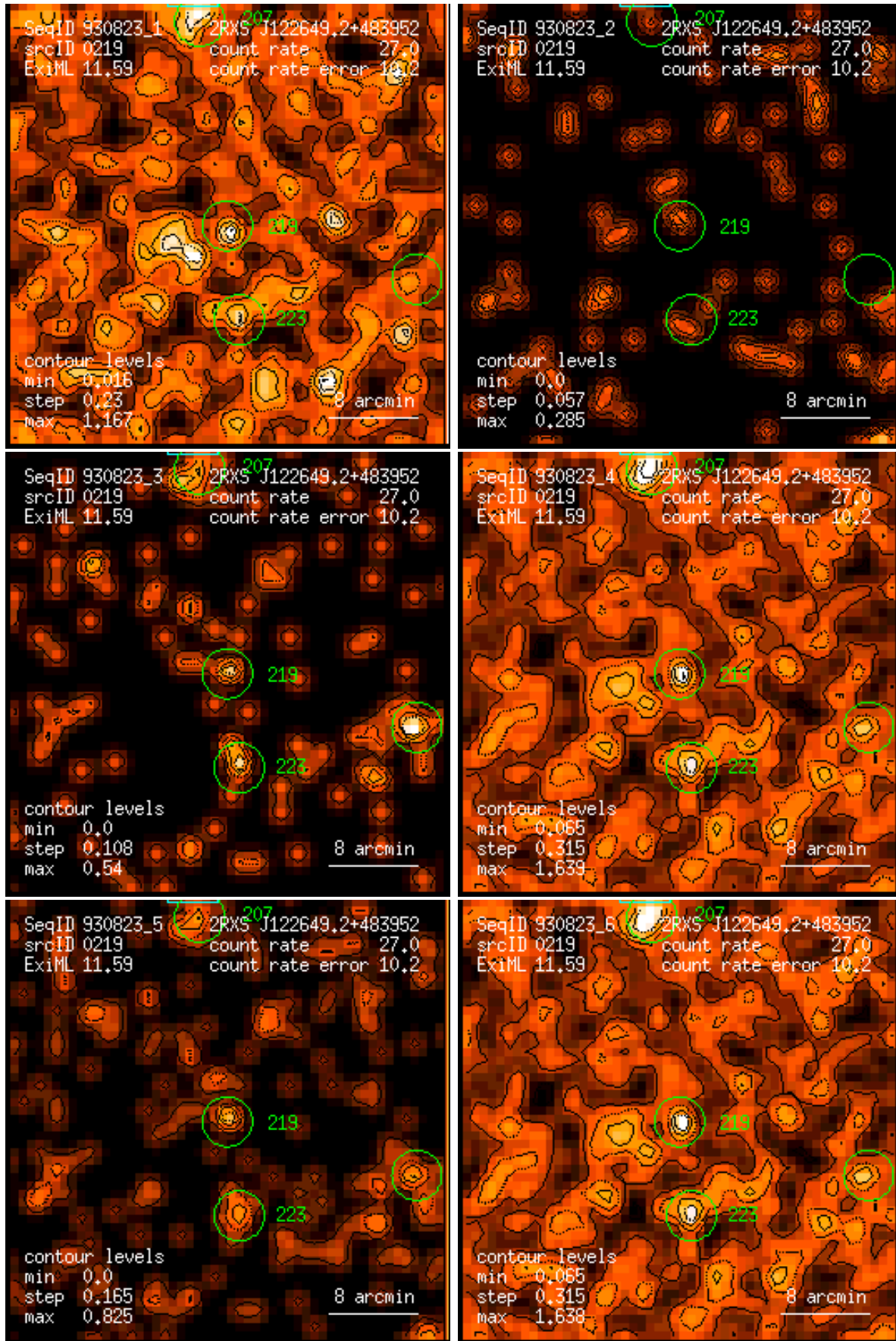
Figure 219: RASS 930823: detection 0219: band rate images, Gaussian filter: (1) PSPC channels 11 – 41, (2) 52 – 90, (3) 91 – 201, (4) 11 – 235, (5) 52 – 201, (6) 11 – 201. Broad band rates in counts/ks. Band rate contour levels in counts/ks/arcmin 2 .
