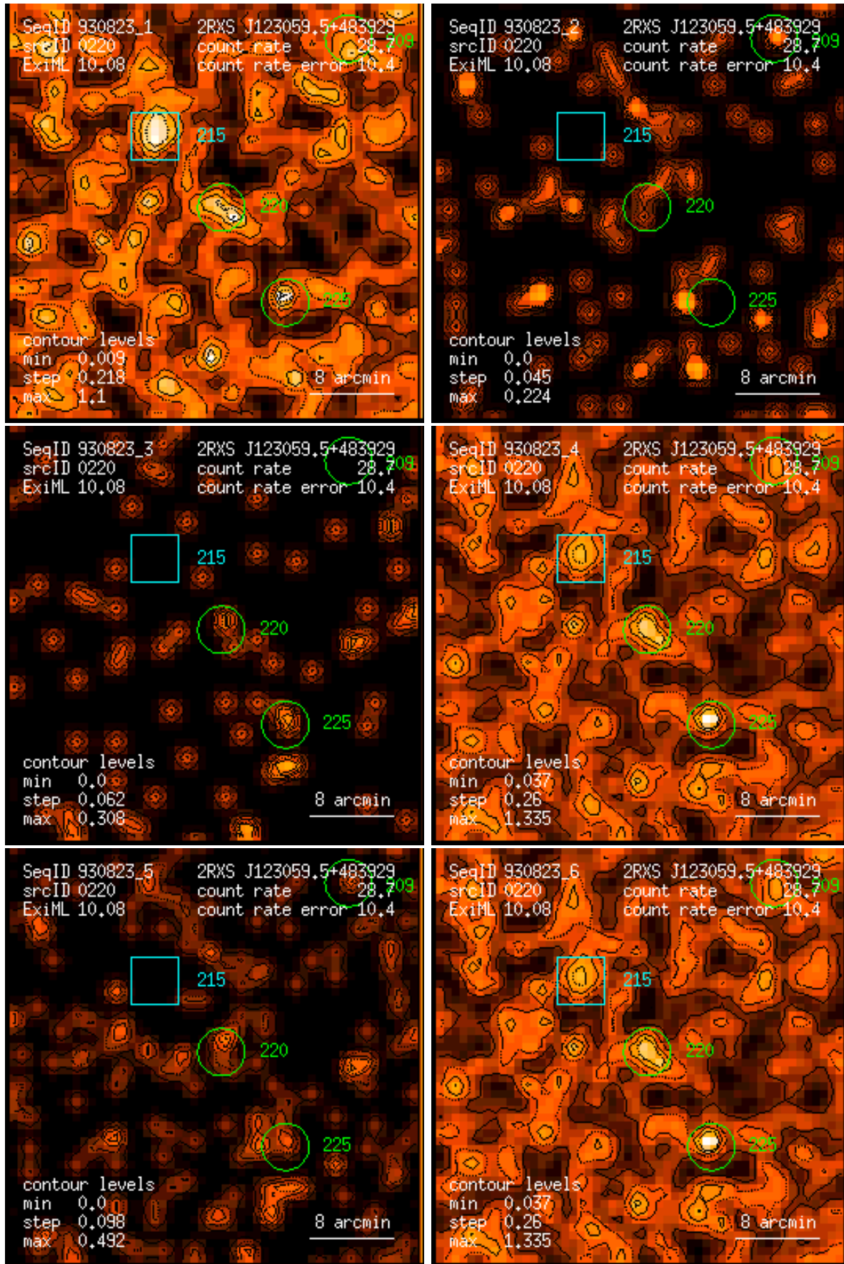
Figure 220: RASS 930823: detection 0220: band rate images, Gaussian filter: (1) PSPC channels 11 – 41, (2) 52 – 90, (3) 91 – 201, (4) 11 – 235, (5) 52 – 201, (6) 11 – 201. Broad band rates in counts/ks. Band rate contour levels in counts/ks/arcmin 2 .
