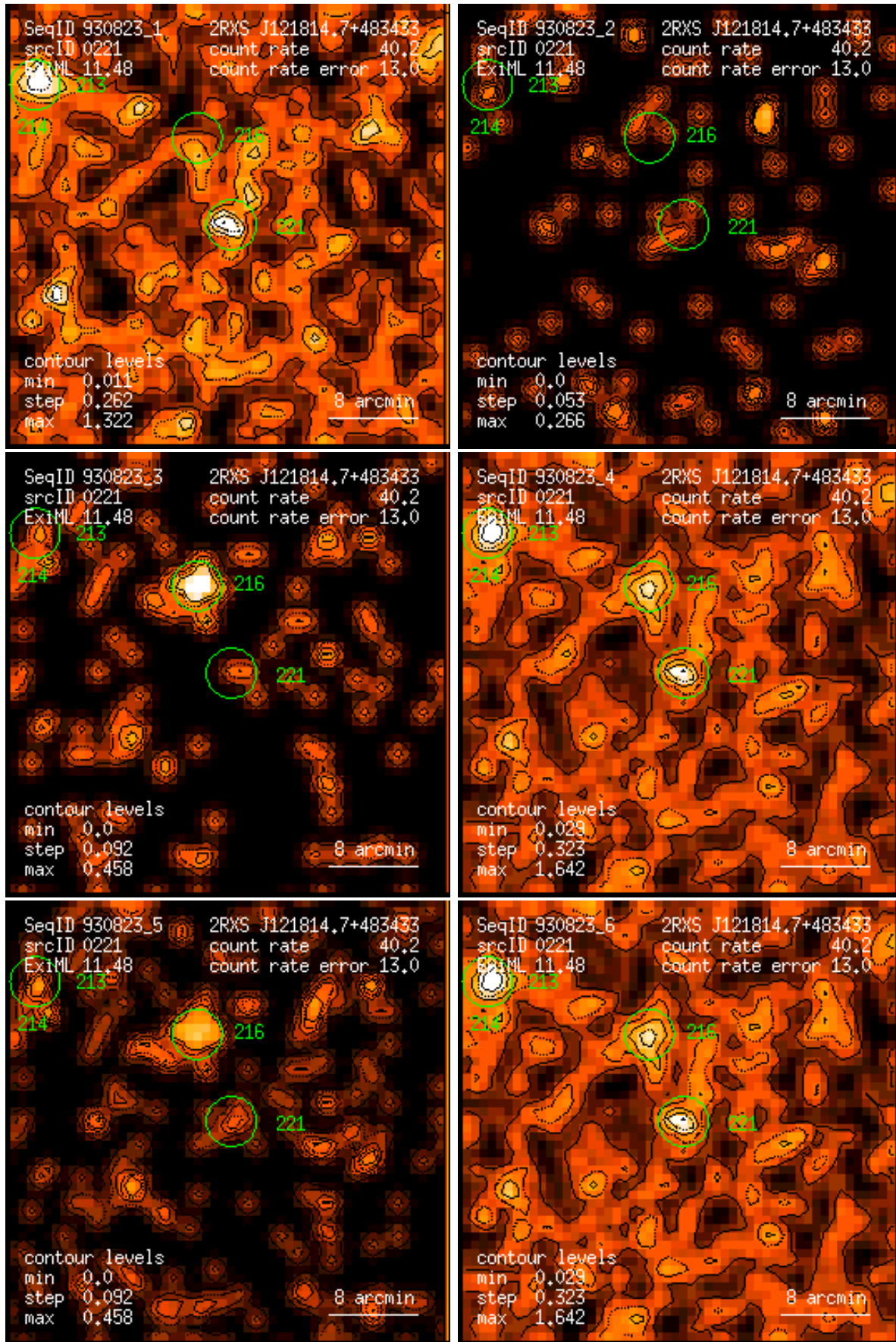
Figure 221: RASS 930823: detection 0221: band rate images, Gaussian filter: (1) PSPC channels 11 – 41, (2) 52 – 90, (3) 91 – 201, (4) 11 – 235, (5) 52 – 201, (6) 11 – 201. Broad band rates in counts/ks. Band rate contour levels in counts/ks/arcmin 2 .
