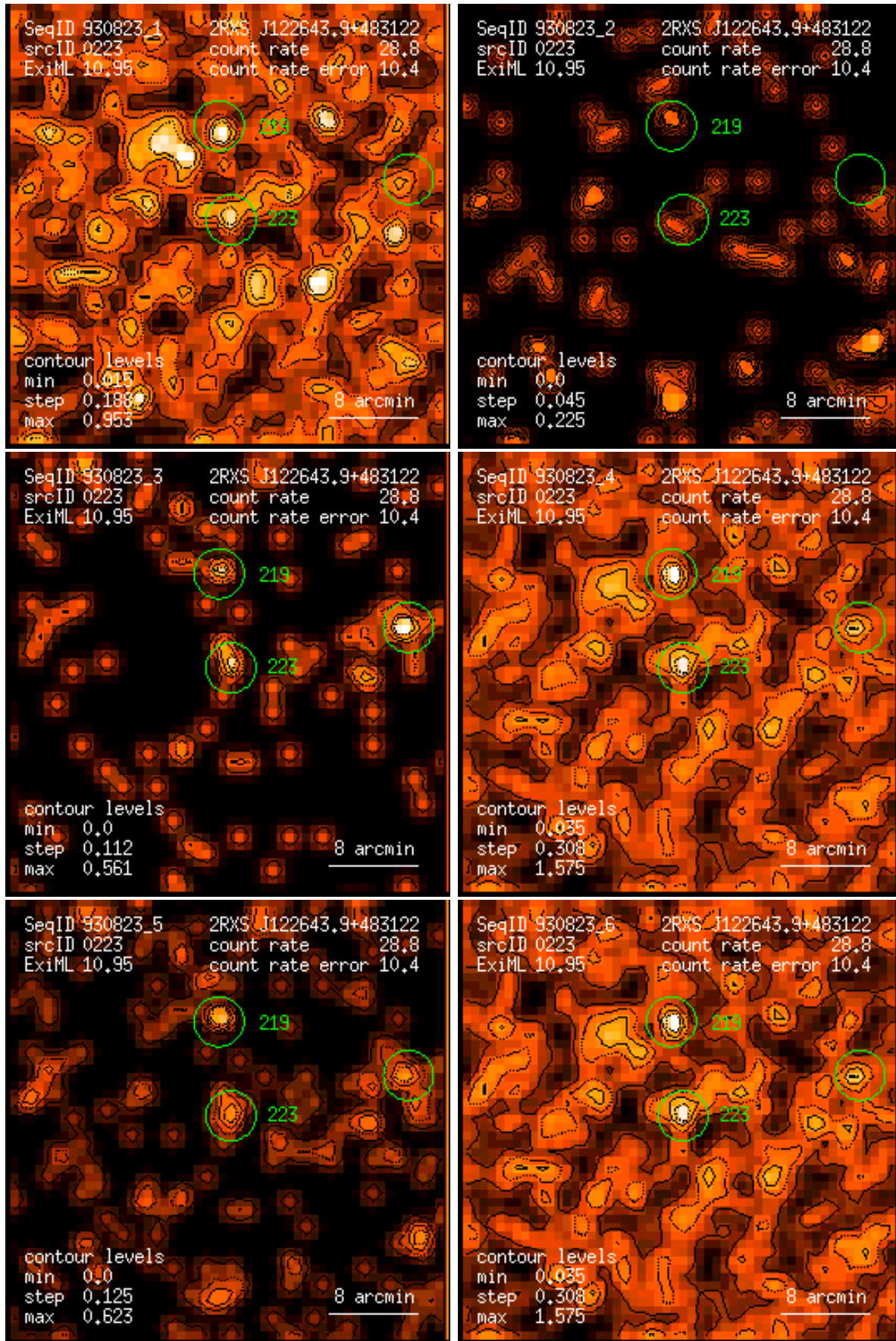
Figure 223: RASS 930823: detection 0223: band rate images, Gaussian filter: (1) PSPC channels 11 – 41, (2) 52 – 90, (3) 91 – 201, (4) 11 – 235, (5) 52 – 201, (6) 11 – 201. Broad band rates in counts/ks. Band rate contour levels in counts/ks/arcmin 2 .
