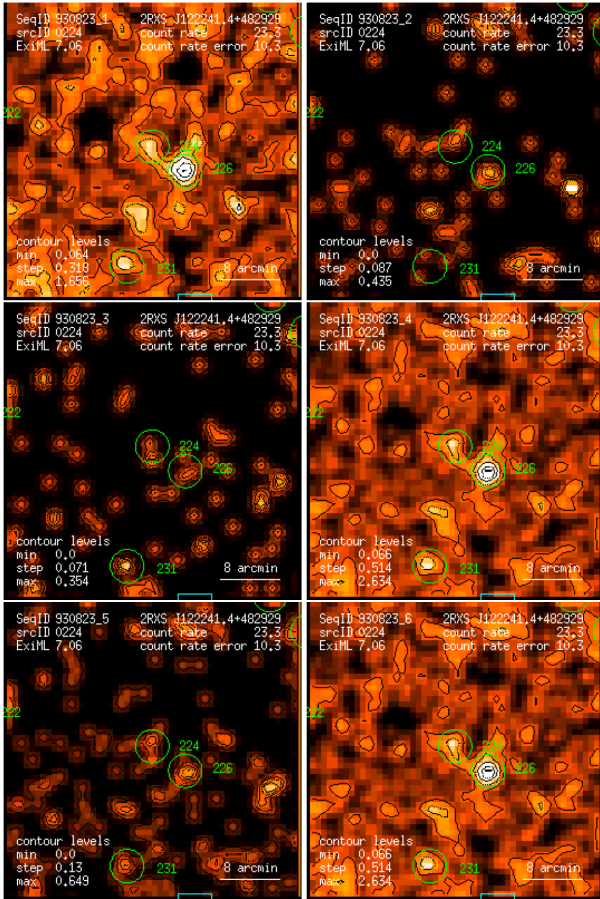
Figure 224: RASS 930823: detection 0224: band rate images, Gaussian filter: (1) PSPC channels 11 – 41, (2) 52 – 90, (3) 91 – 201, (4) 11 – 235, (5) 52 – 201, (6) 11 – 201. Broad band rates in counts/ks. Band rate contour levels in counts/ks/arcmin 2 .
