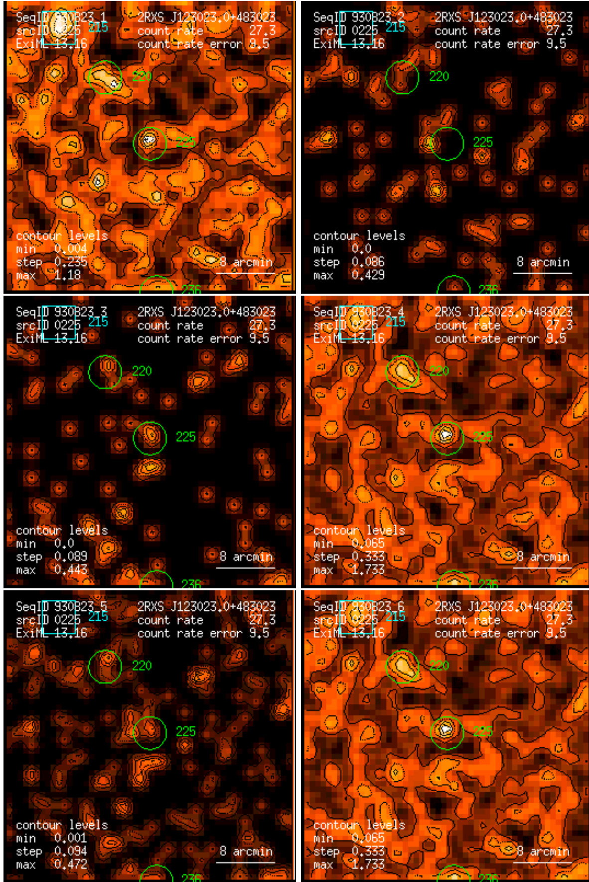
Figure 225: RASS 930823: detection 0225: band rate images, Gaussian filter: (1) PSPC channels 11 – 41, (2) 52 – 90, (3) 91 – 201, (4) 11 – 235, (5) 52 – 201, (6) 11 – 201. Broad band rates in counts/ks. Band rate contour levels in counts/ks/arcmin 2 .
