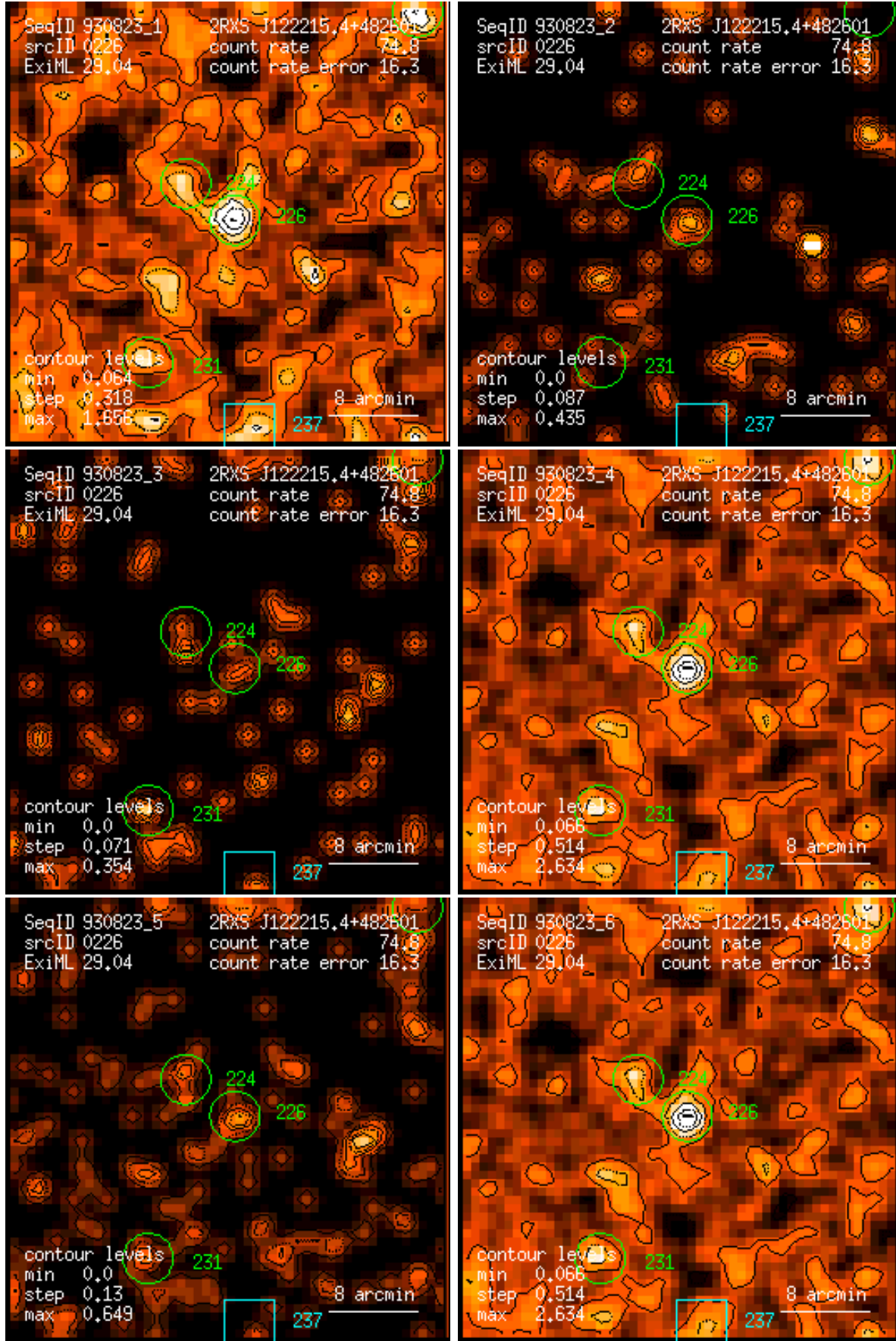
Figure 226: RASS 930823: detection 0226: band rate images, Gaussian filter: (1) PSPC channels 11 – 41, (2) 52 – 90, (3) 91 – 201, (4) 11 – 235, (5) 52 – 201, (6) 11 – 201. Broad band rates in counts/ks. Band rate contour levels in counts/ks/arcmin 2 .
