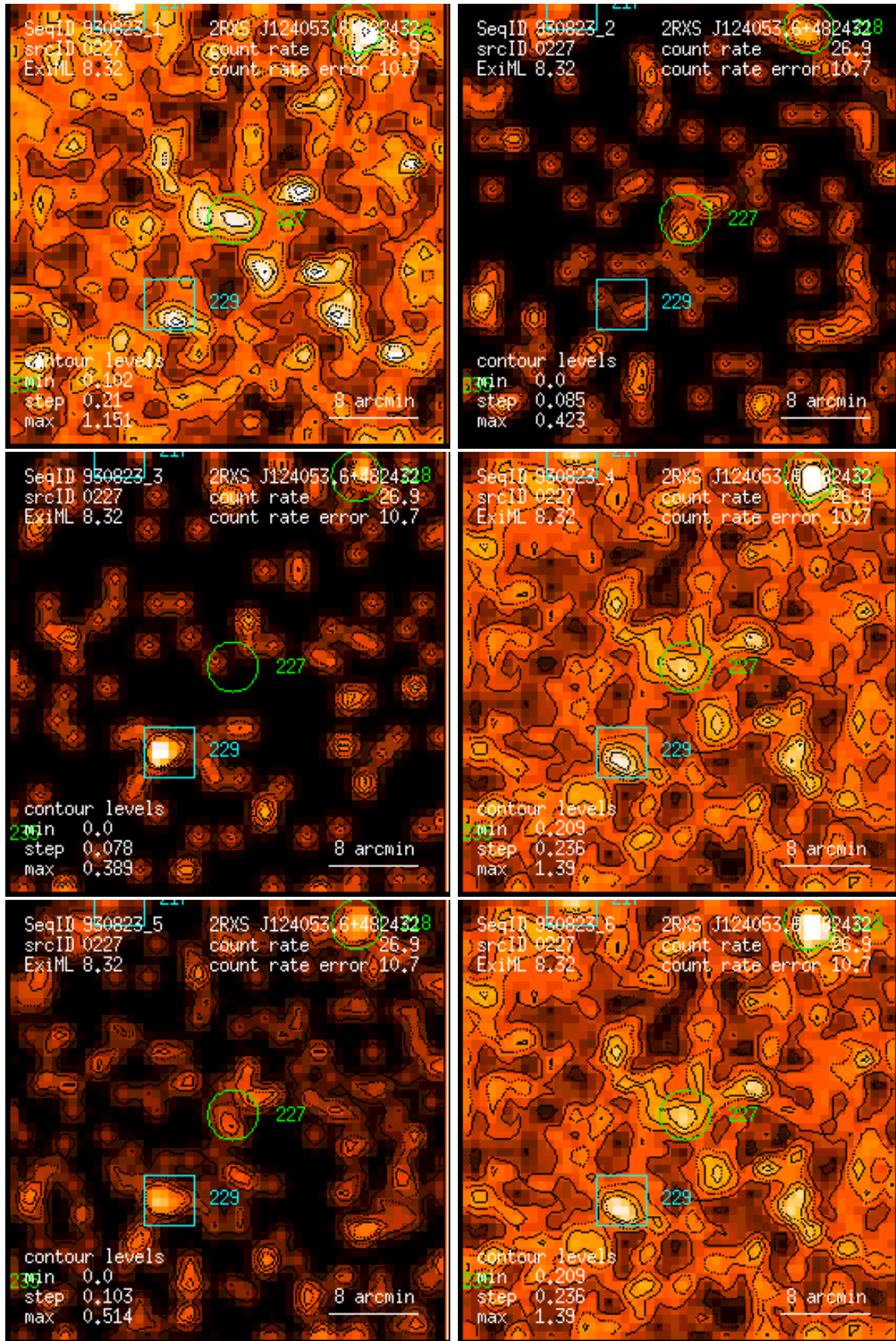
Figure 227: RASS 930823: detection 0227: band rate images, Gaussian filter: (1) PSPC channels 11 – 41, (2) 52 – 90, (3) 91 – 201, (4) 11 – 235, (5) 52 – 201, (6) 11 – 201. Broad band rates in counts/ks. Band rate contour levels in counts/ks/arcmin 2 .
