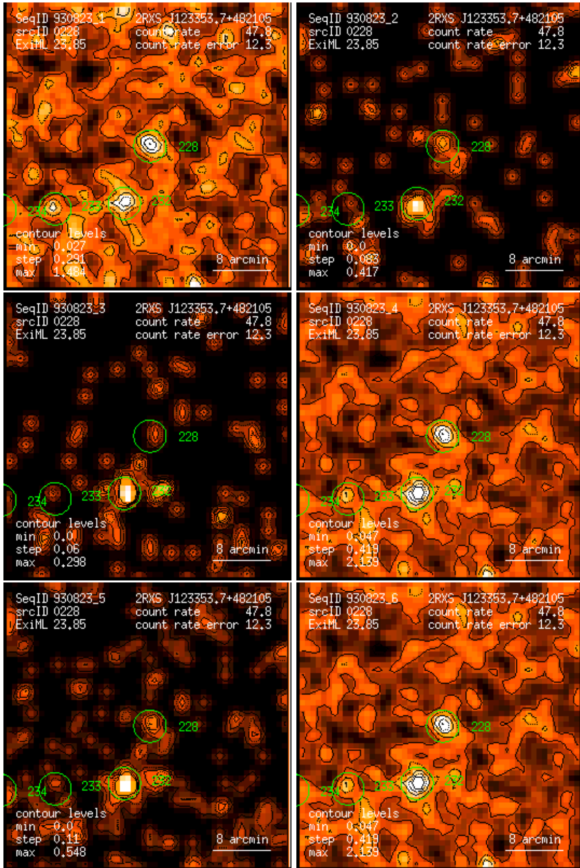
Figure 228: RASS 930823: detection 0228: band rate images, Gaussian filter: (1) PSPC channels 11 – 41, (2) 52 – 90, (3) 91 – 201, (4) 11 – 235, (5) 52 – 201, (6) 11 – 201. Broad band rates in counts/ks. Band rate contour levels in counts/ks/arcmin 2 .
