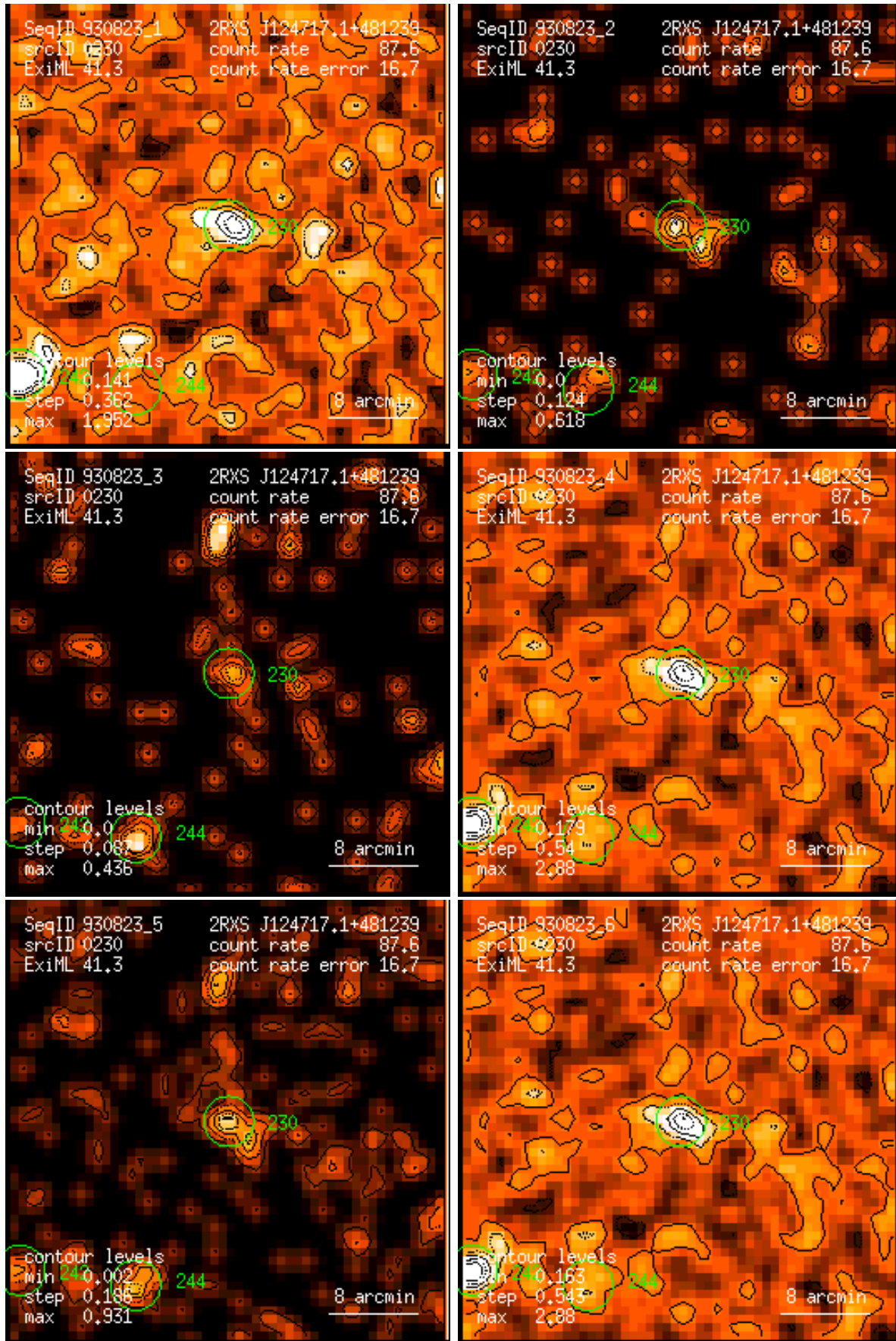
Figure 230: RASS 930823: detection 0230: band rate images, Gaussian filter: (1) PSPC channels 11 – 41, (2) 52 – 90, (3) 91 – 201, (4) 11 – 235, (5) 52 – 201, (6) 11 – 201. Broad band rates in counts/ks. Band rate contour levels in counts/ks/arcmin 2 .
