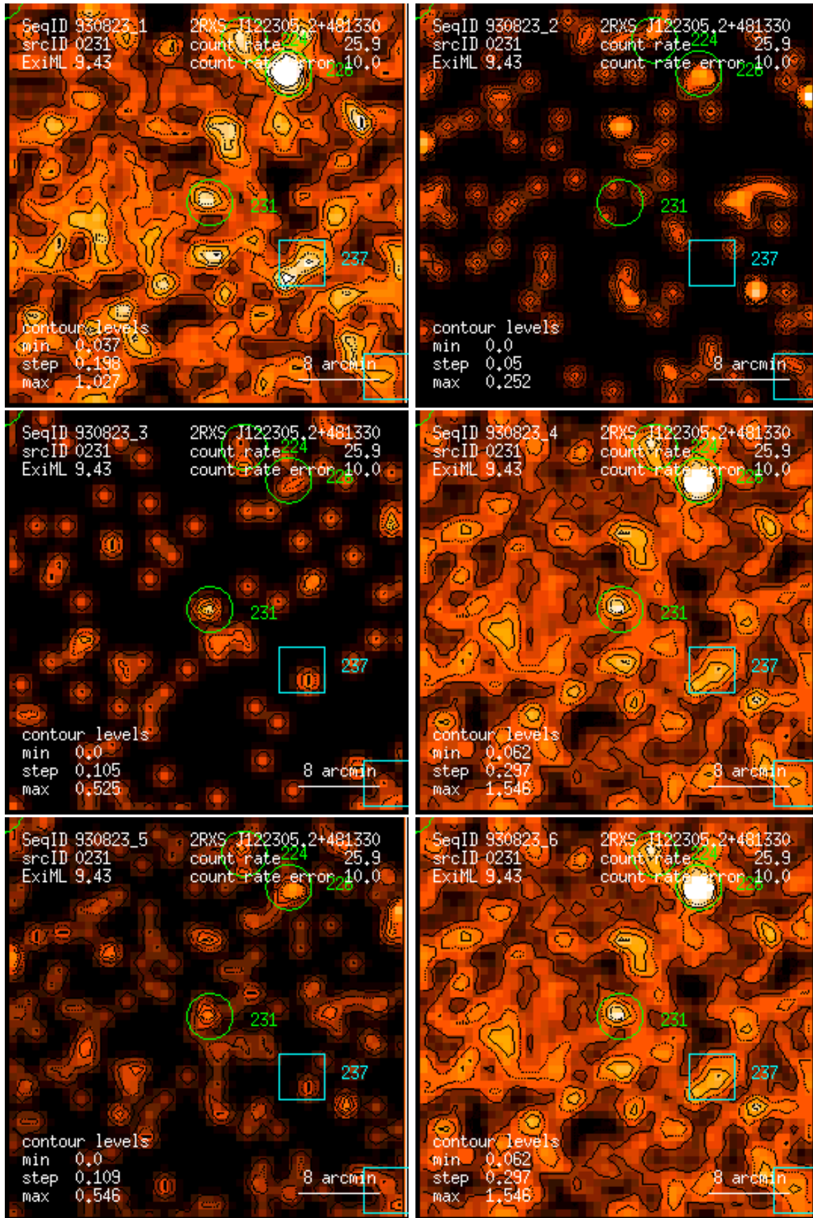
Figure 231: RASS 930823: detection 0231: band rate images, Gaussian filter: (1) PSPC channels 11 – 41, (2) 52 – 90, (3) 91 – 201, (4) 11 – 235, (5) 52 – 201, (6) 11 – 201. Broad band rates in counts/ks. Band rate contour levels in counts/ks/arcmin 2 .
