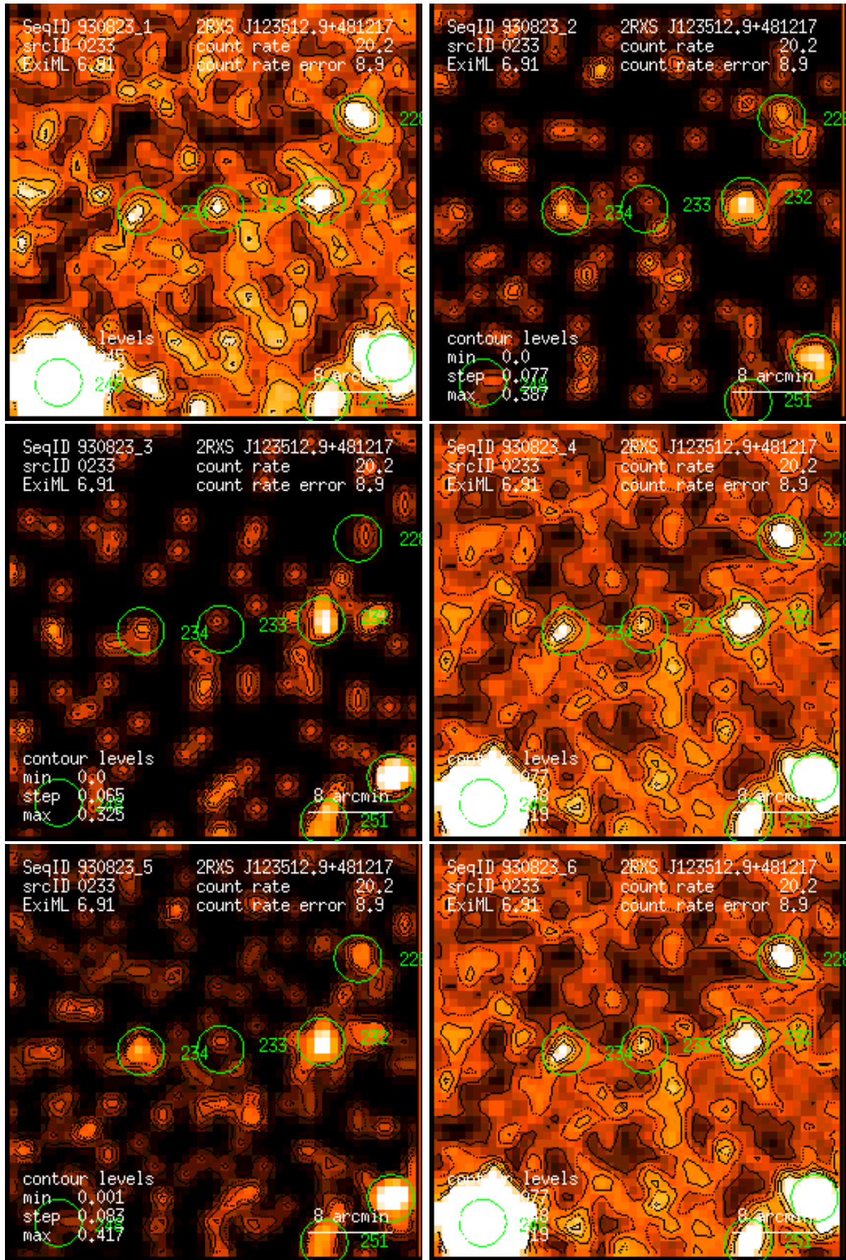
Figure 233: RASS 930823: detection 0233: band rate images, Gaussian filter: (1) PSPC channels 11 – 41, (2) 52 – 90, (3) 91 – 201, (4) 11 – 235, (5) 52 – 201, (6) 11 – 201. Broad band rates in counts/ks. Band rate contour levels in counts/ks/arcmin 2 .
