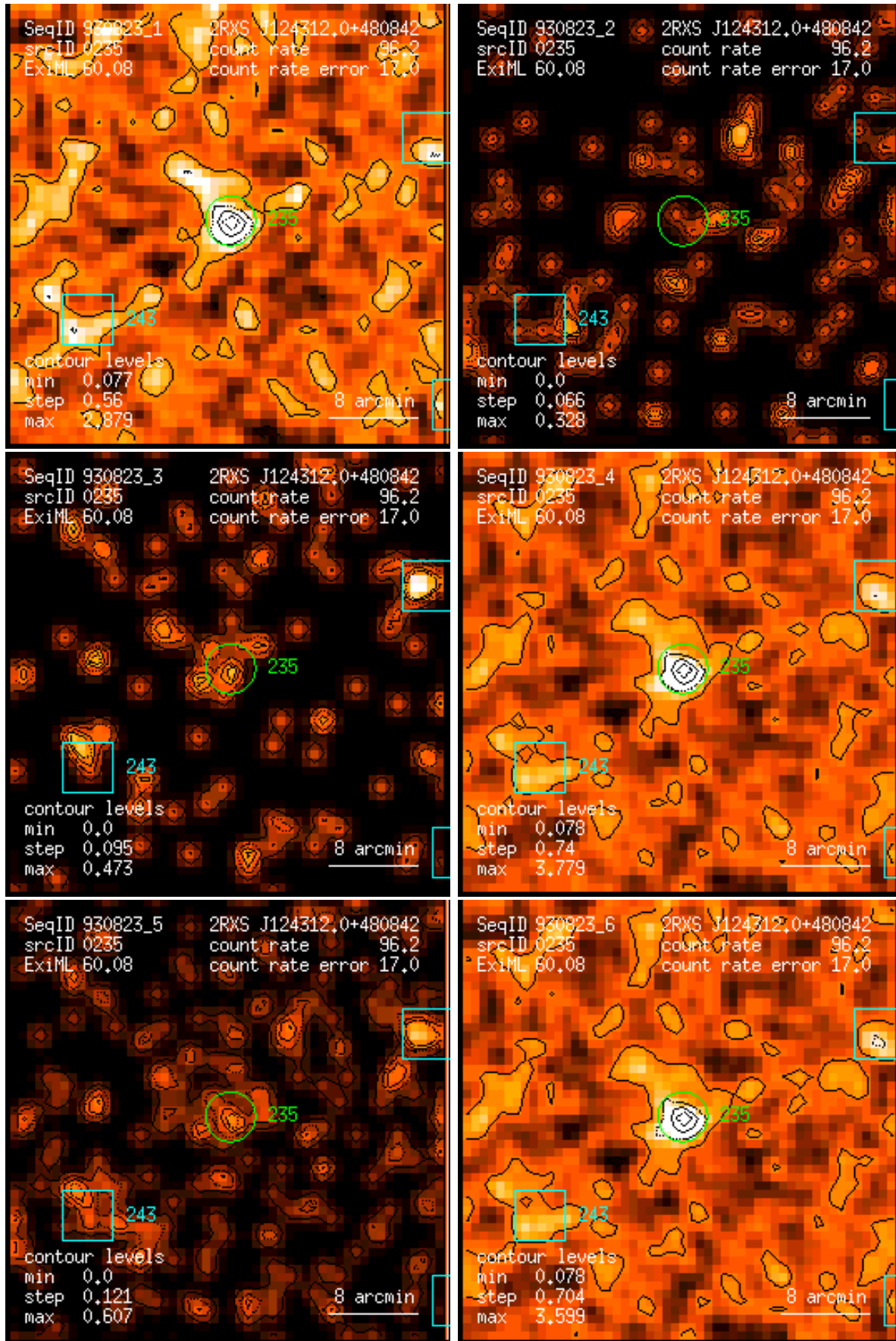
Figure 235: RASS 930823: detection 0235: band rate images, Gaussian filter: (1) PSPC channels 11 – 41, (2) 52 – 90, (3) 91 – 201, (4) 11 – 235, (5) 52 – 201, (6) 11 – 201. Broad band rates in counts/ks. Band rate contour levels in counts/ks/arcmin 2 .
