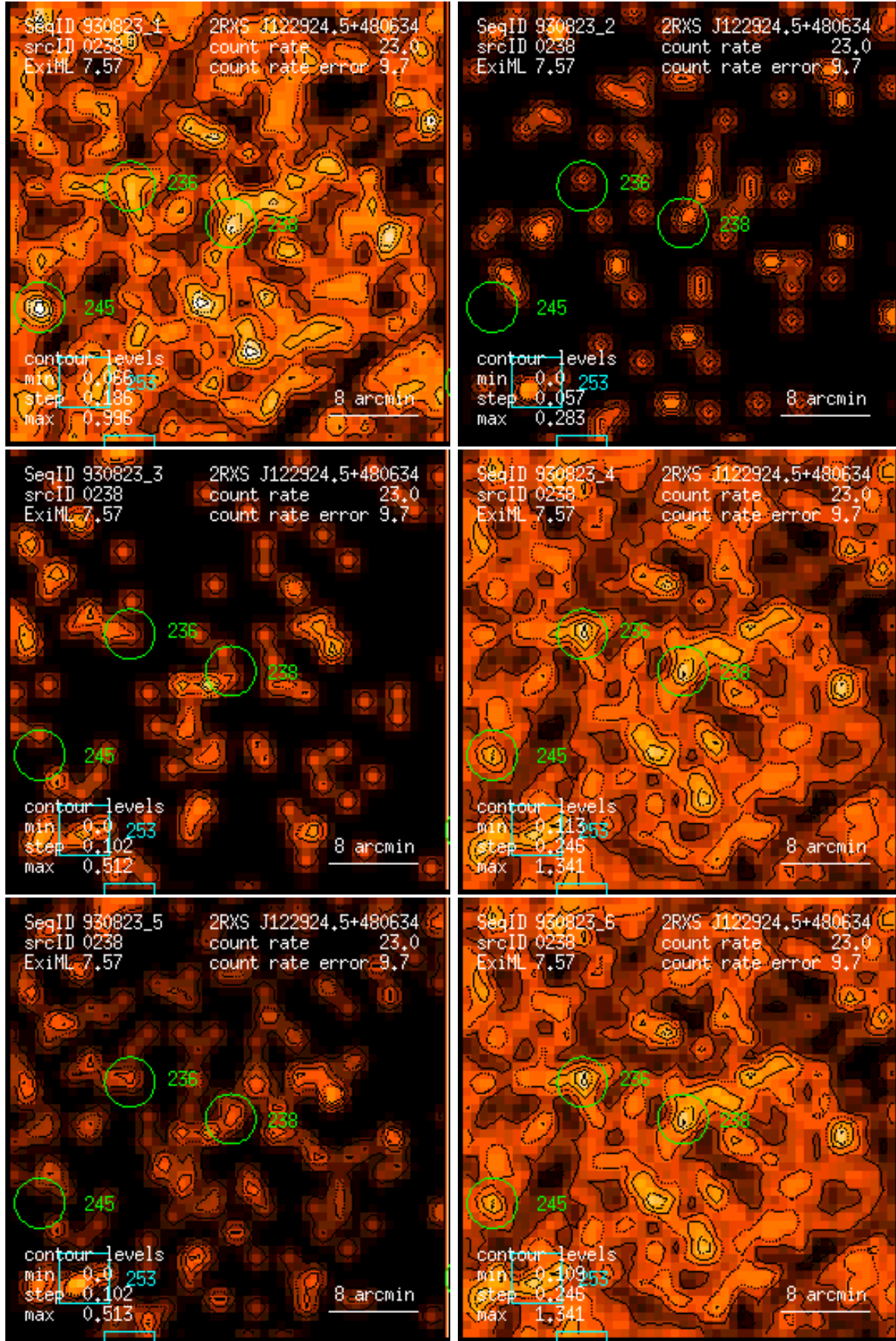
Figure 238: RASS 930823: detection 0238: band rate images, Gaussian filter: (1) PSPC channels 11 – 41, (2) 52 – 90, (3) 91 – 201, (4) 11 – 235, (5) 52 – 201, (6) 11 – 201. Broad band rates in counts/ks. Band rate contour levels in counts/ks/arcmin 2 .
