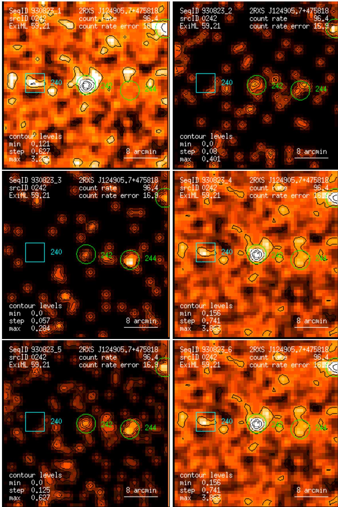
Figure 242: RASS 930823: detection 0242: band rate images, Gaussian filter: (1) PSPC channels 11 – 41, (2) 52 – 90, (3) 91 – 201, (4) 11 – 235, (5) 52 – 201, (6) 11 – 201. Broad band rates in counts/ks. Band rate contour levels in counts/ks/arcmin 2 .
