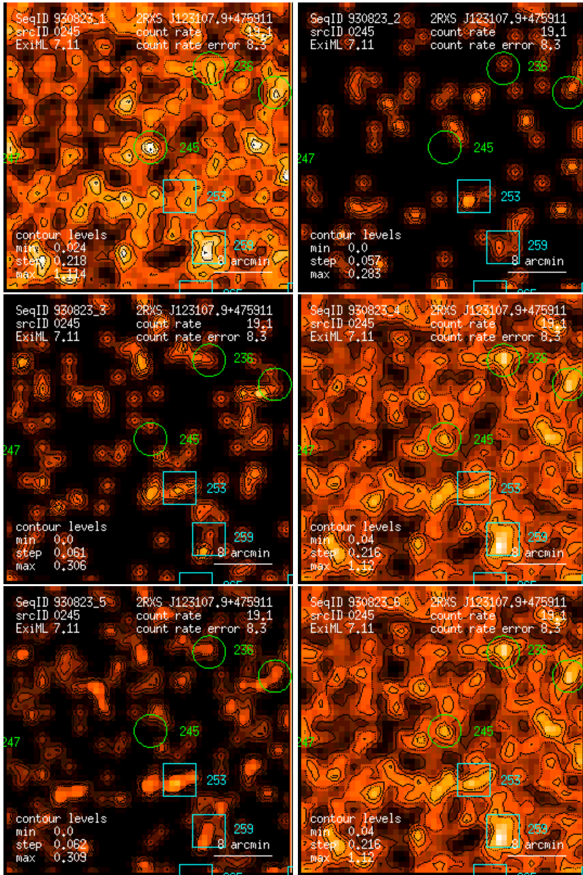
Figure 245: RASS 930823: detection 0245: band rate images, Gaussian filter: (1) PSPC channels 11 – 41, (2) 52 – 90, (3) 91 – 201, (4) 11 – 235, (5) 52 – 201, (6) 11 – 201. Broad band rates in counts/ks. Band rate contour levels in counts/ks/arcmin 2 .
