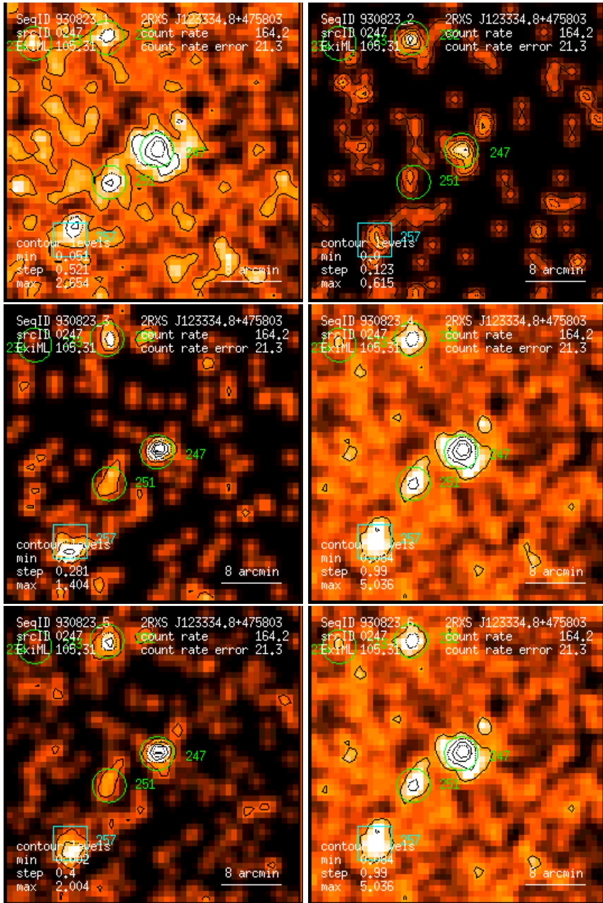
Figure 247: RASS 930823: detection 0247: band rate images, Gaussian filter: (1) PSPC channels 11 – 41, (2) 52 – 90, (3) 91 – 201, (4) 11 – 235, (5) 52 – 201, (6) 11 – 201. Broad band rates in counts/ks. Band rate contour levels in counts/ks/arcmin 2 .
