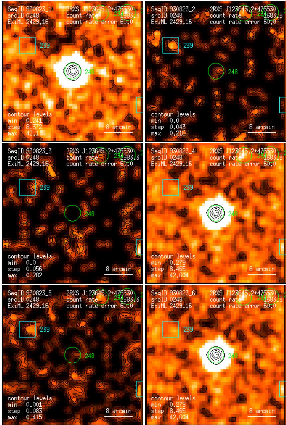
Figure 248: RASS 930823: detection 0248: band rate images, Gaussian filter: (1) PSPC channels 11 – 41, (2) 52 – 90, (3) 91 – 201, (4) 11 – 235, (5) 52 – 201, (6) 11 – 201. Broad band rates in counts/ks. Band rate contour levels in counts/ks/arcmin 2 .
