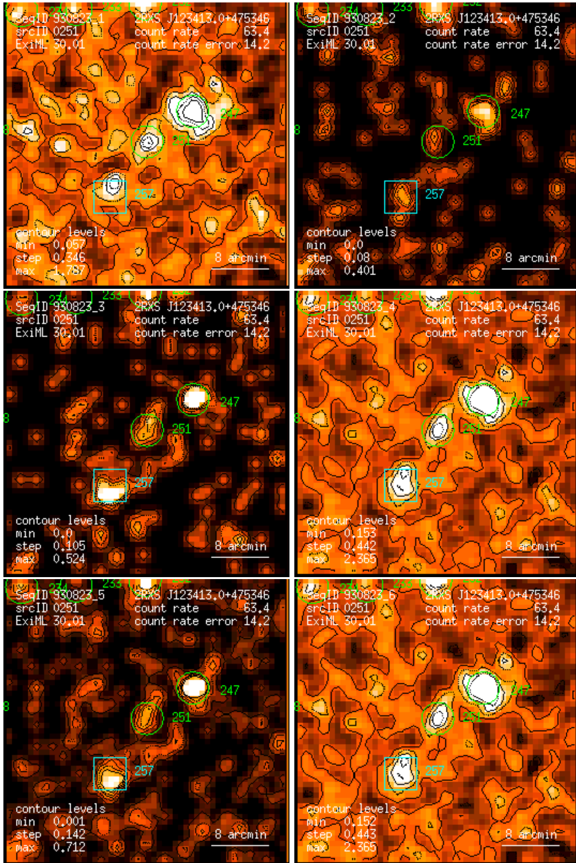
Figure 251: RASS 930823: detection 0251: band rate images, Gaussian filter: (1) PSPC channels 11 – 41, (2) 52 – 90, (3) 91 – 201, (4) 11 – 235, (5) 52 – 201, (6) 11 – 201. Broad band rates in counts/ks. Band rate contour levels in counts/ks/arcmin 2 .
