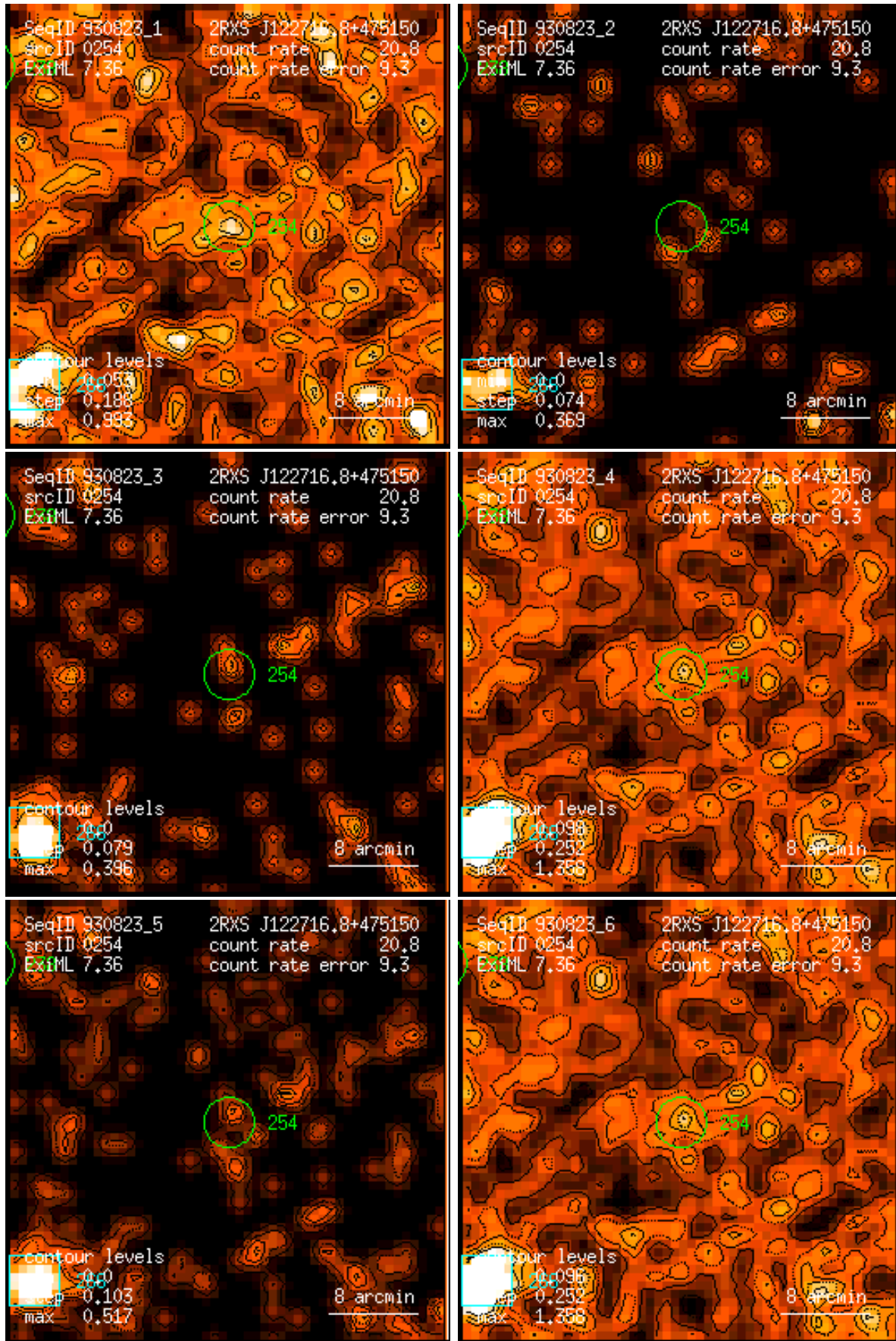
Figure 254: RASS 930823: detection 0254: band rate images, Gaussian filter: (1) PSPC channels 11 – 41, (2) 52 – 90, (3) 91 – 201, (4) 11 – 235, (5) 52 – 201, (6) 11 – 201. Broad band rates in counts/ks. Band rate contour levels in counts/ks/arcmin 2 .
