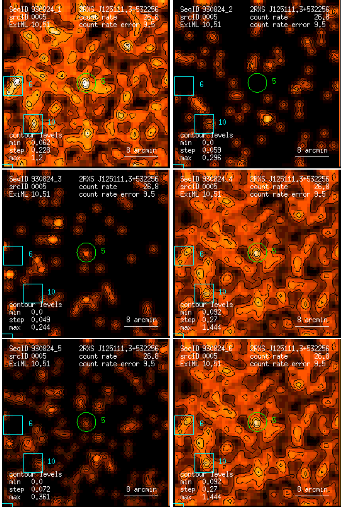
Figure 5: RASS 930824: detection 0005: band rate images, Gaussian filter: (1) PSPC channels 11 – 41, (2) 52 – 90, (3) 91 – 201, (4) 11 – 235, (5) 52 – 201, (6) 11 – 201. Broad band rates in counts/ks. Band rate contour levels in counts/ks/arcmin 2 .
