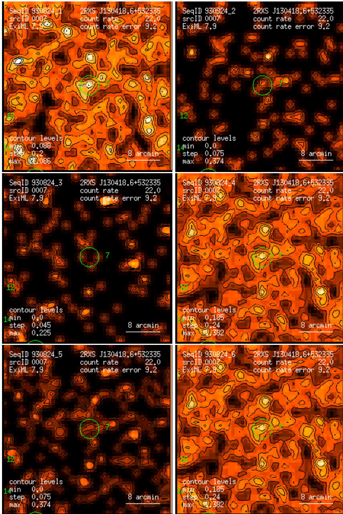
Figure 7: RASS 930824: detection 0007: band rate images, Gaussian filter: (1) PSPC channels 11 – 41, (2) 52 – 90, (3) 91 – 201, (4) 11 – 235, (5) 52 – 201, (6) 11 – 201. Broad band rates in counts/ks. Band rate contour levels in counts/ks/arcmin 2 .
