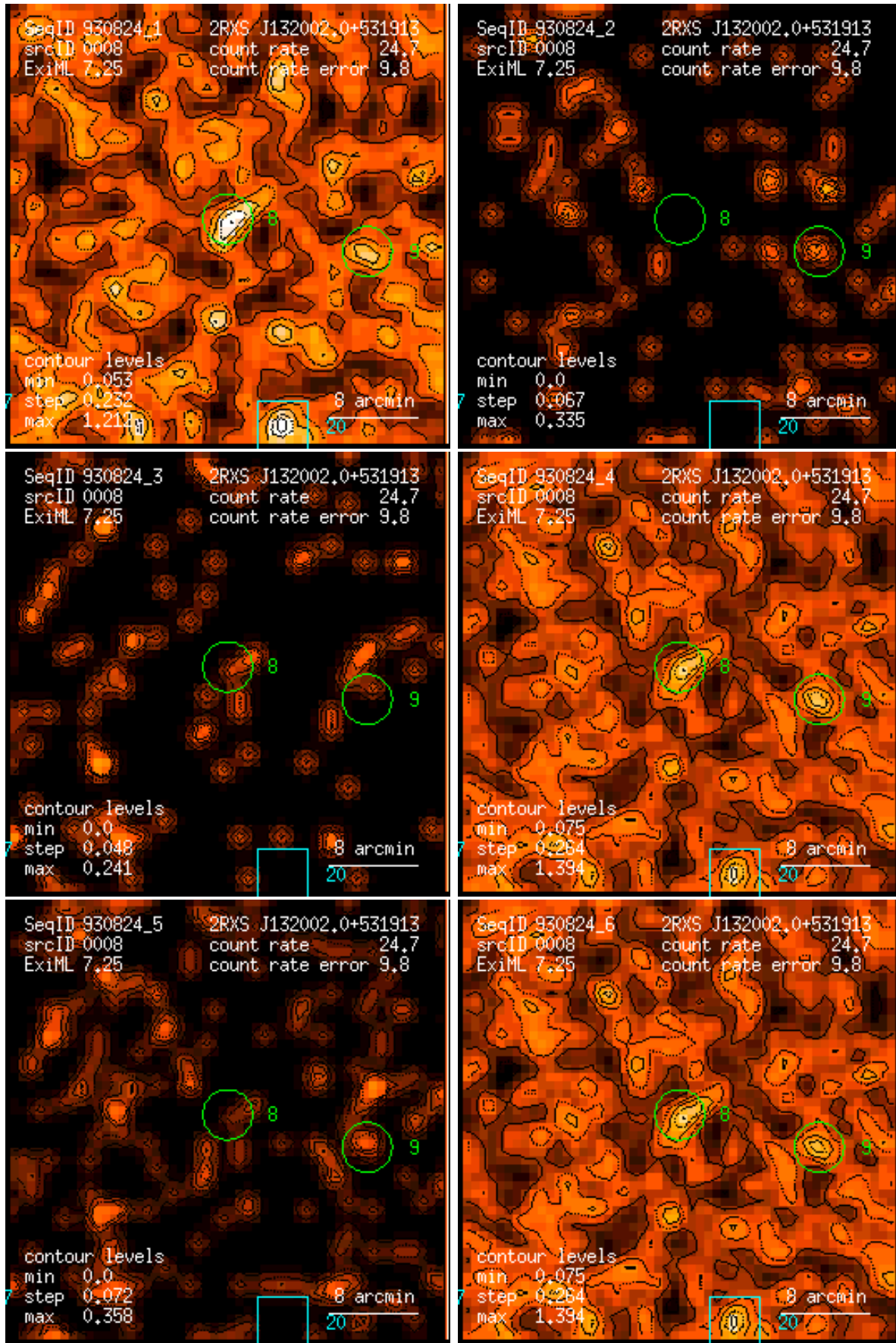
Figure 8: RASS 930824: detection 0008: band rate images, Gaussian filter: (1) PSPC channels 11 – 41, (2) 52 – 90, (3) 91 – 201, (4) 11 – 235, (5) 52 – 201, (6) 11 – 201. Broad band rates in counts/ks. Band rate contour levels in counts/ks/arcmin 2 .
