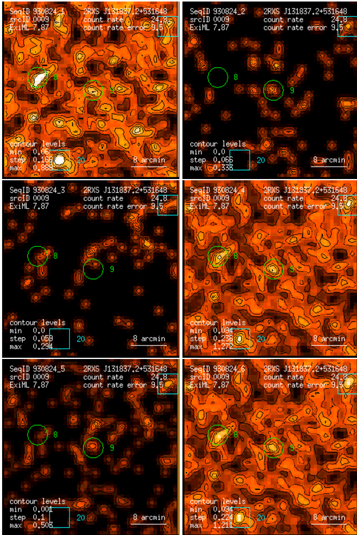
Figure 9: RASS 930824: detection 0009: band rate images, Gaussian filter: (1) PSPC channels 11 – 41, (2) 52 – 90, (3) 91 – 201, (4) 11 – 235, (5) 52 – 201, (6) 11 – 201. Broad band rates in counts/ks. Band rate contour levels in counts/ks/arcmin 2 .
