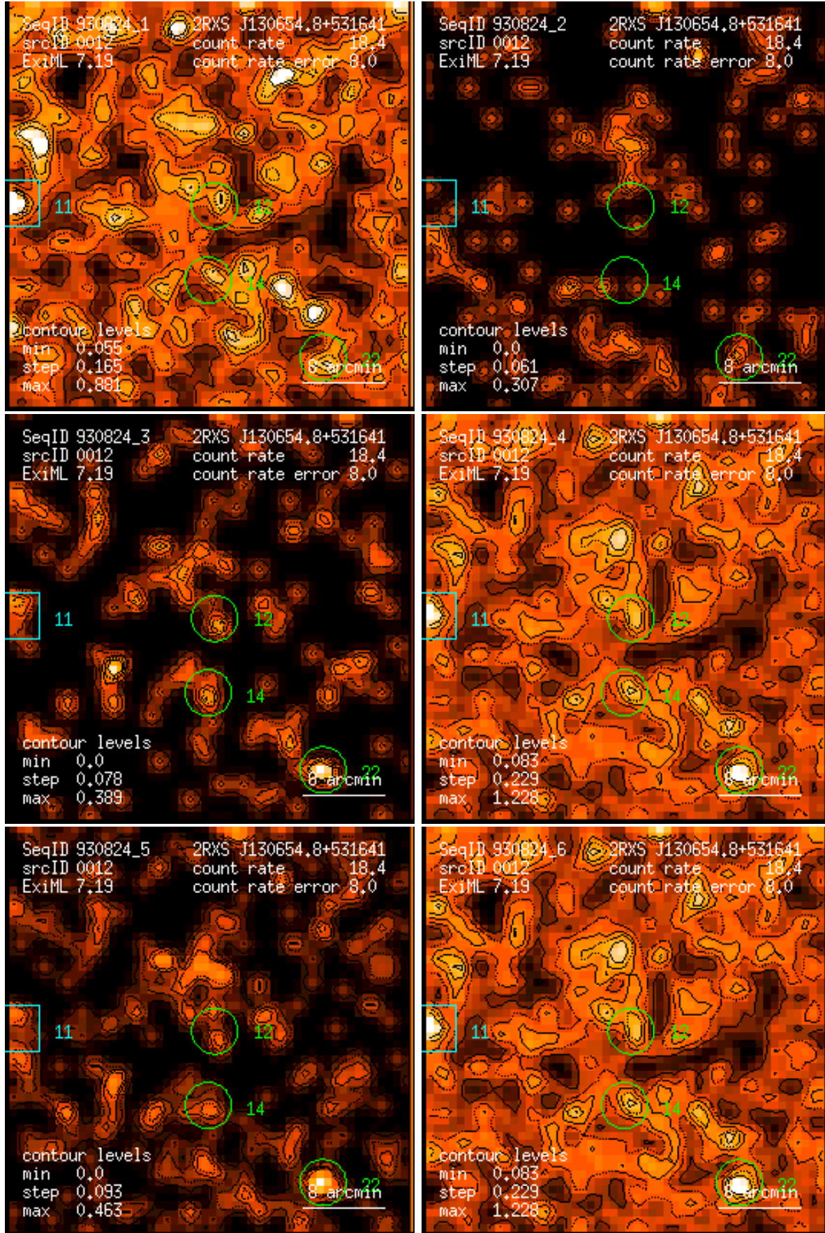
Figure 12: RASS 930824: detection 0012: band rate images, Gaussian filter: (1) PSPC channels 11 – 41, (2) 52 – 90, (3) 91 – 201, (4) 11 – 235, (5) 52 – 201, (6) 11 – 201. Broad band rates in counts/ks. Band rate contour levels in counts/ks/arcmin 2 .
