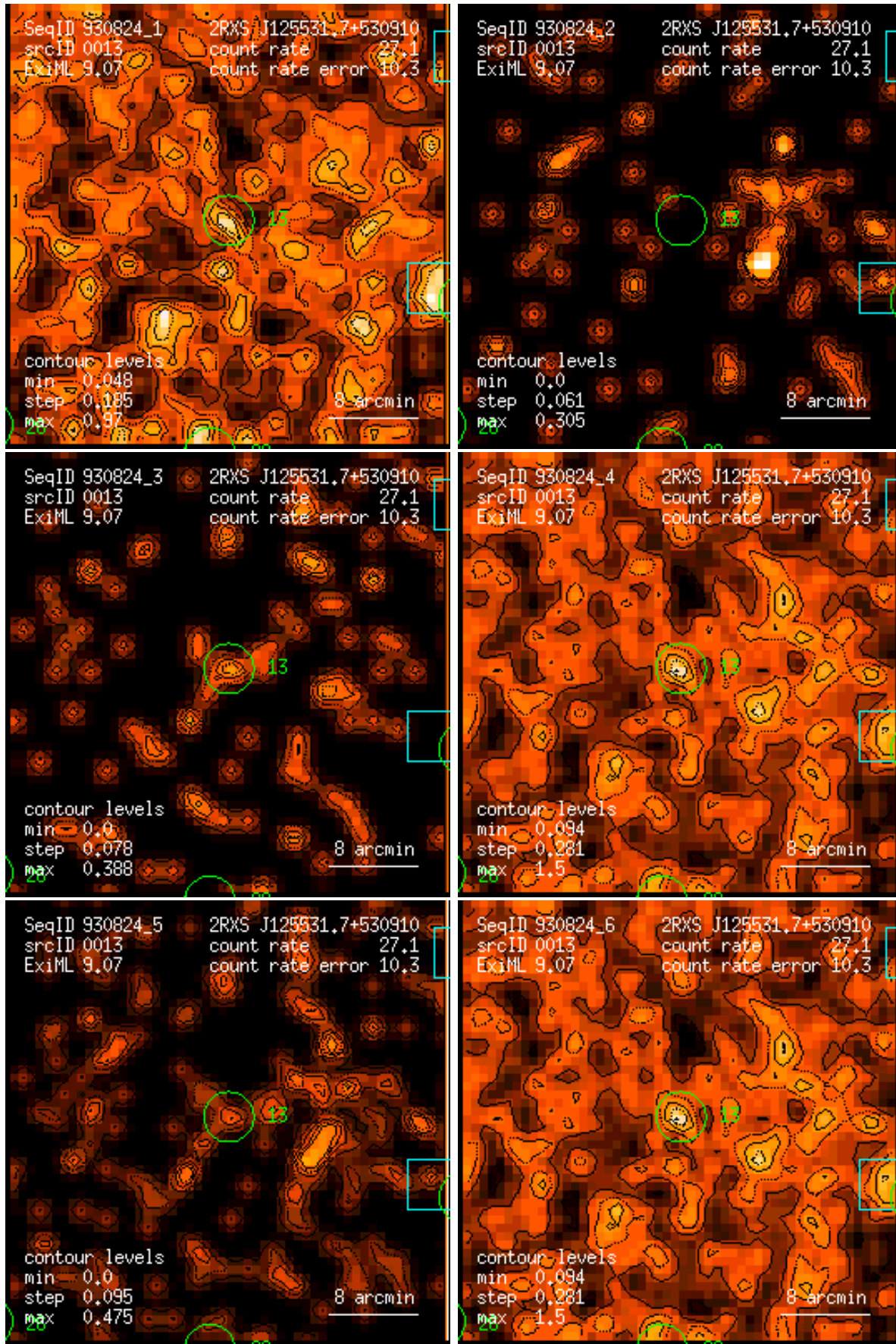
Figure 13: RASS 930824: detection 0013: band rate images, Gaussian filter: (1) PSPC channels 11 – 41, (2) 52 – 90, (3) 91 – 201, (4) 11 – 235, (5) 52 – 201, (6) 11 – 201. Broad band rates in counts/ks. Band rate contour levels in counts/ks/arcmin 2 .
