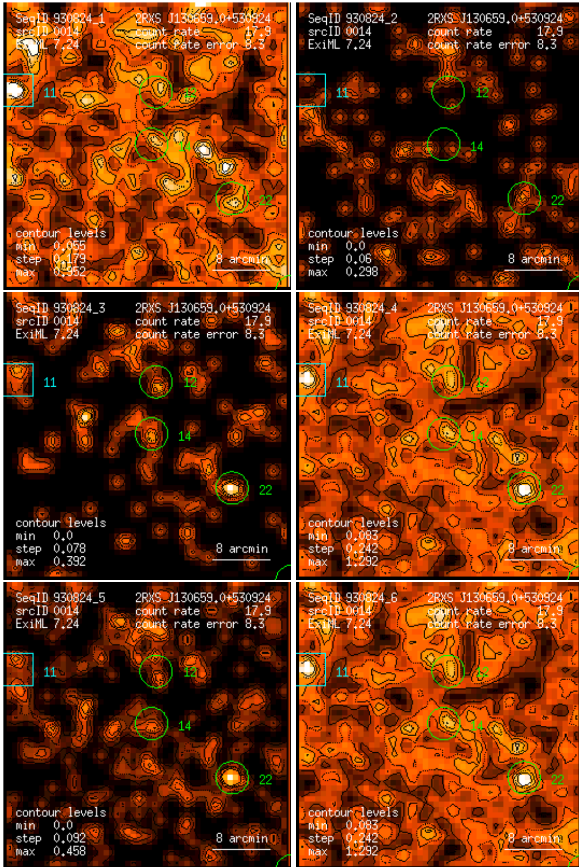
Figure 14: RASS 930824: detection 0014: band rate images, Gaussian filter: (1) PSPC channels 11 – 41, (2) 52 – 90, (3) 91 – 201, (4) 11 – 235, (5) 52 – 201, (6) 11 – 201. Broad band rates in counts/ks. Band rate contour levels in counts/ks/arcmin 2 .
