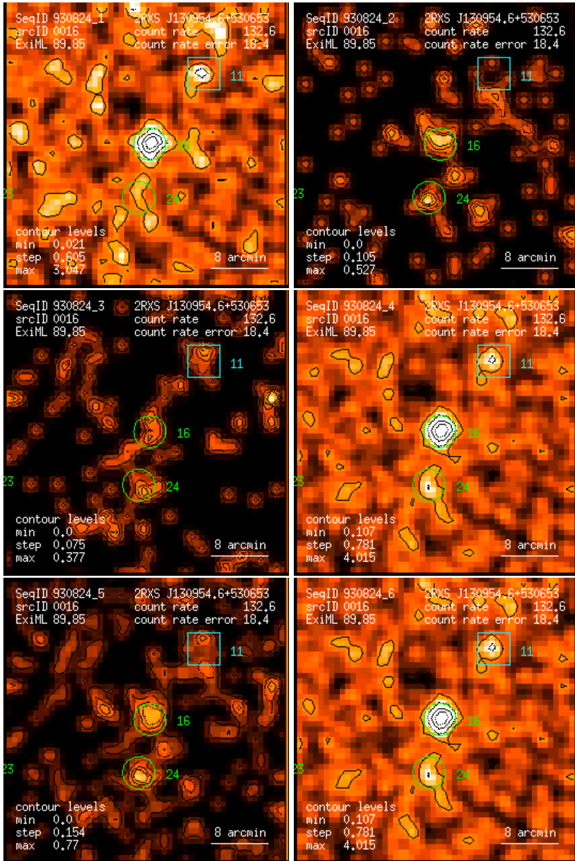
Figure 16: RASS 930824: detection 0016: band rate images, Gaussian filter: (1) PSPC channels 11 – 41, (2) 52 – 90, (3) 91 – 201, (4) 11 – 235, (5) 52 – 201, (6) 11 – 201. Broad band rates in counts/ks. Band rate contour levels in counts/ks/arcmin 2 .
